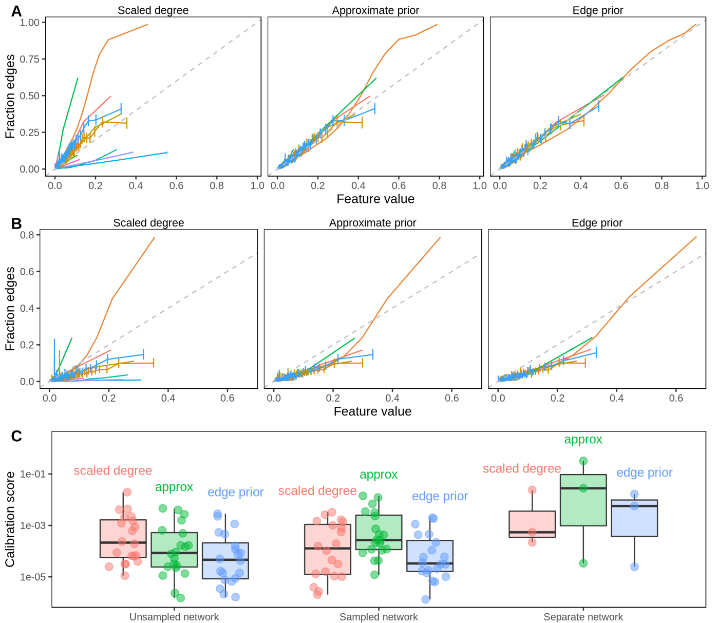
Figure 6: The edge prior accurately assigns the probability of edge existence. A. Calibration curves for full network reconstruction of 20 networks from Hetinet. For every unique predictor value on the horizontal axis, the fraction of node pairs with that predictor value having an edge in the network is shown on the vertical axis. The permutation-based edge prior's calibration was superior to the other two strategies based on degree. B. Calibration curves for sampled network reconstruction. The edge prior shows superior calibration in the 20 Hetinet networks. C. Individual Hetinet edge type calibration estimated by the two-component decomposition of the Brier score, in which lower scores indicate better calibration. The edge prior has excellent calibration in unsampled and sampled networks, and each considered method is sensitive to shifts in the degree distribution.
