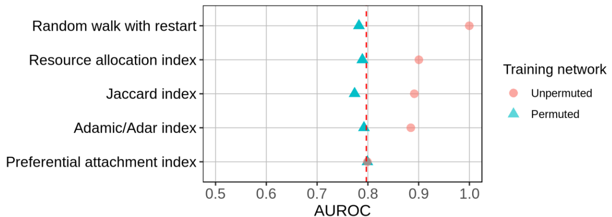
Figure 9: Identifying the fraction of a metric’s performance resulting from degree alone. Network reconstruction performances by five edge prediction features. Dotted red line indicates performance of the edge prior. Each feature was computed on both the unpermuted and 100 permutations of the STRING PPI network.
