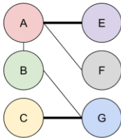
Figure 3: Modified XSwap algorithm graphical explanation.
