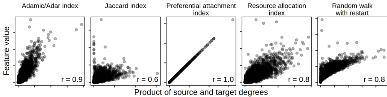
Figure 8: Common edge-prediction metrics correlate with node degree. Five common edge-prediction features (Supplemental Table 2) are correlated with node degree on the STRING PPI network [24]. All five features show a positive relationship with degree, though the magnitude of this correlation is highly variable. The preferential attachment index is understandably perfectly correlated because it is equal to the product of source and target degree. Each panel indicates the Pearson correlation (“r”) between feature and degree in the lower right corner.
