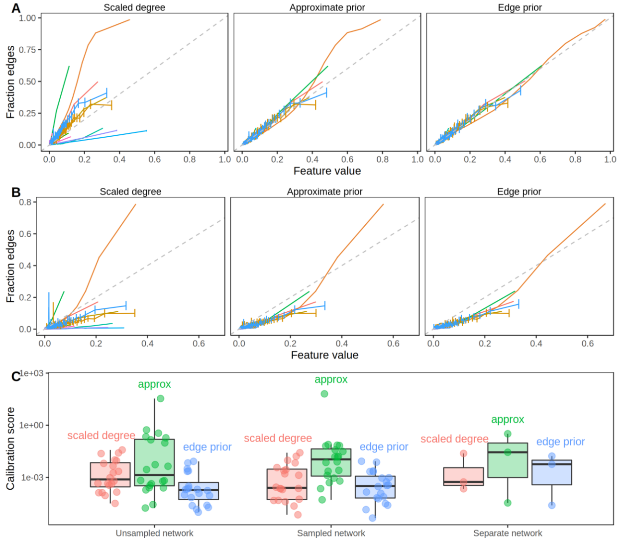
Figure 7: The edge prior accurately assigns the probability of edge existence. A.
