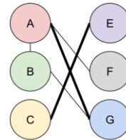
Figure 3: Modified XSwap algorithm graphical explanation.
