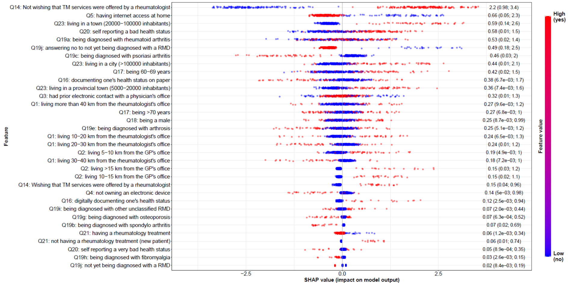
Figure S3: Feature importance according to SHAP values – no vs. not answered/do not know classification
