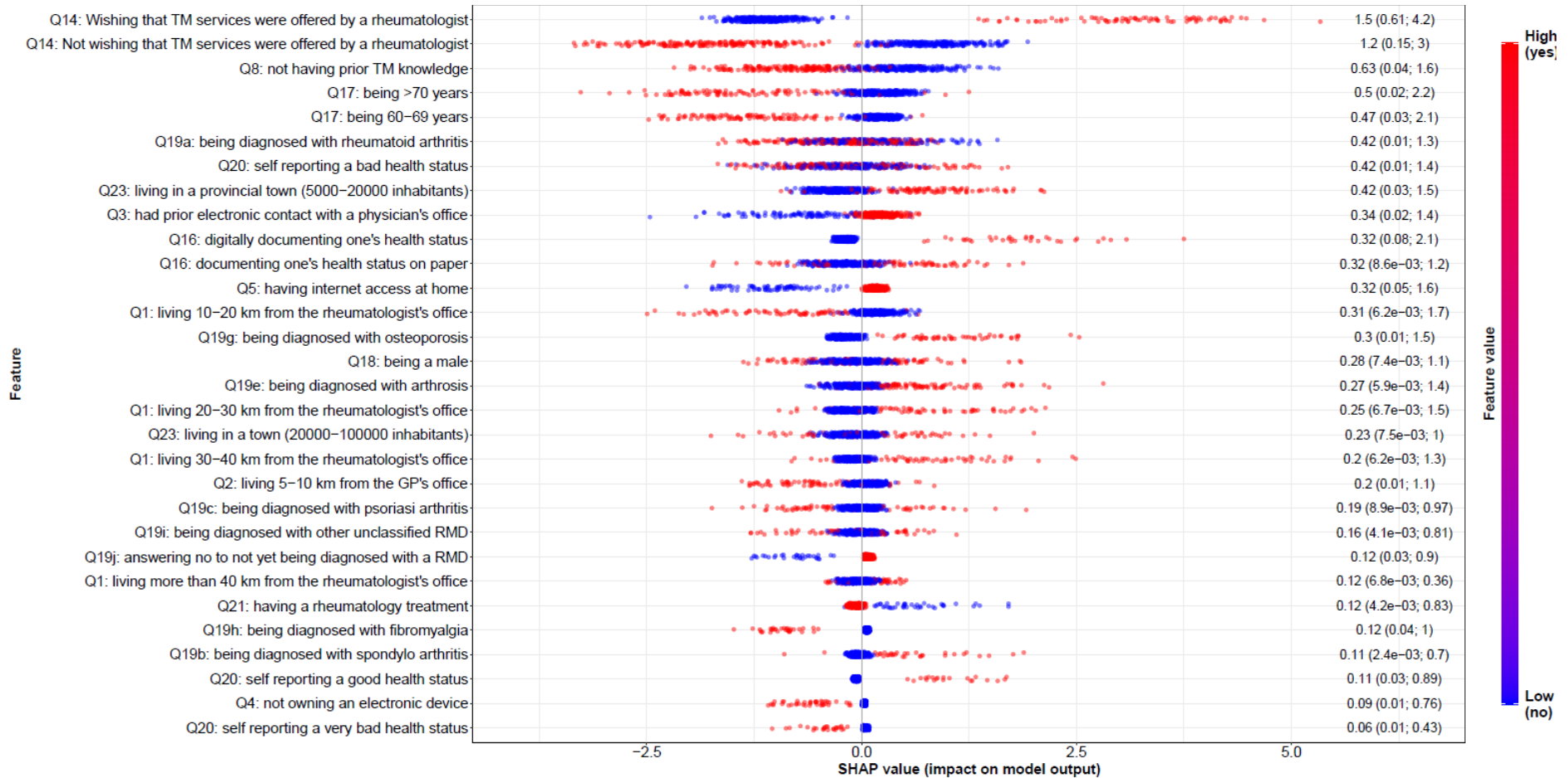
Figure S4: Feature importance according to SHAP values – yes vs. rest classification
