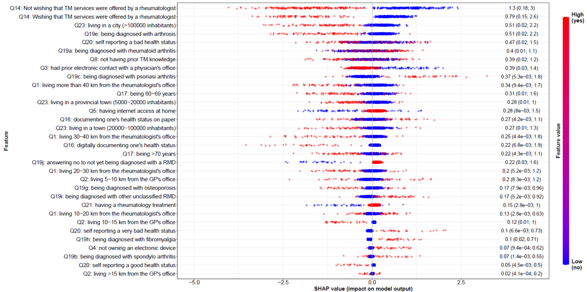
Figure S6: Feature importance according to SHAP values – not answered/do not know vs. rest classification
