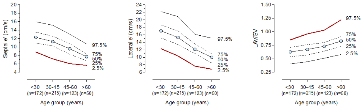
Figure S2. Age-specific percentiles of diastolic function indexes from 560 healthy references. The red line represents low-risk reference cut-offs for reference limits.
