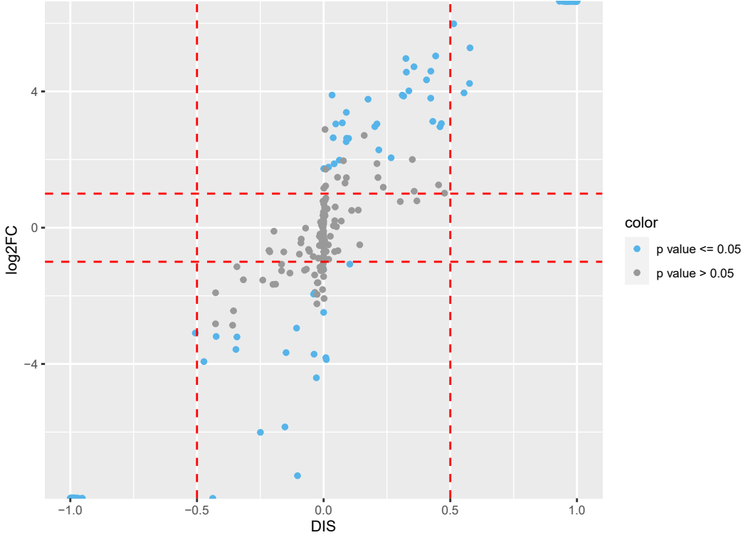
Scatter plot of DIS vs. log2FC (NT/RNase+)
