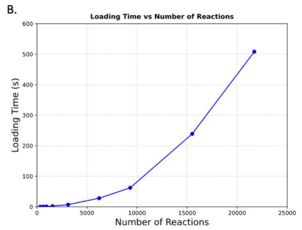
S1 Fig. Simulation and Loading time of ODE Models Increases as the Number of Reactions in the Model Increase.
