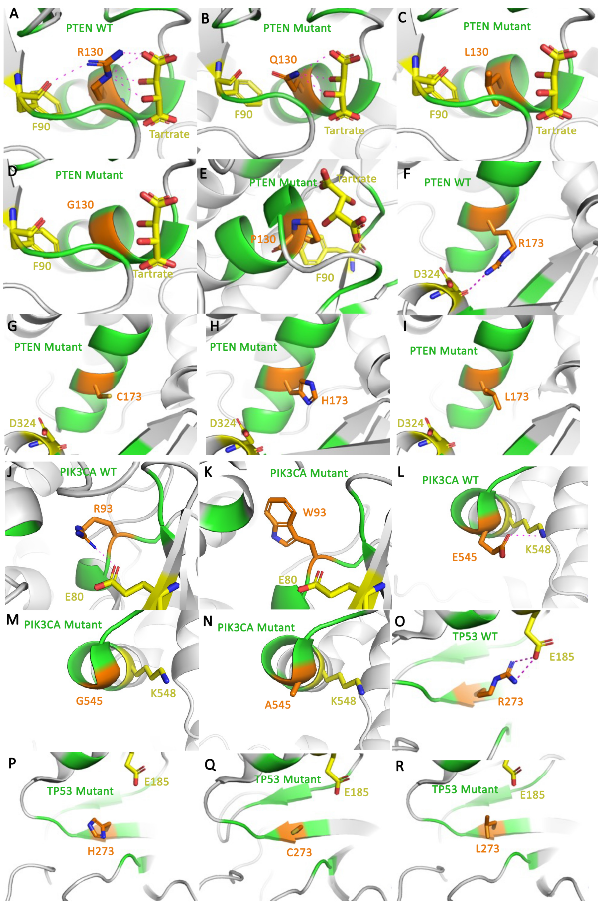
Supplemental Figure S4. Comparison of WT and mutant structures where a reduction in tertiary polar interactions was observed
