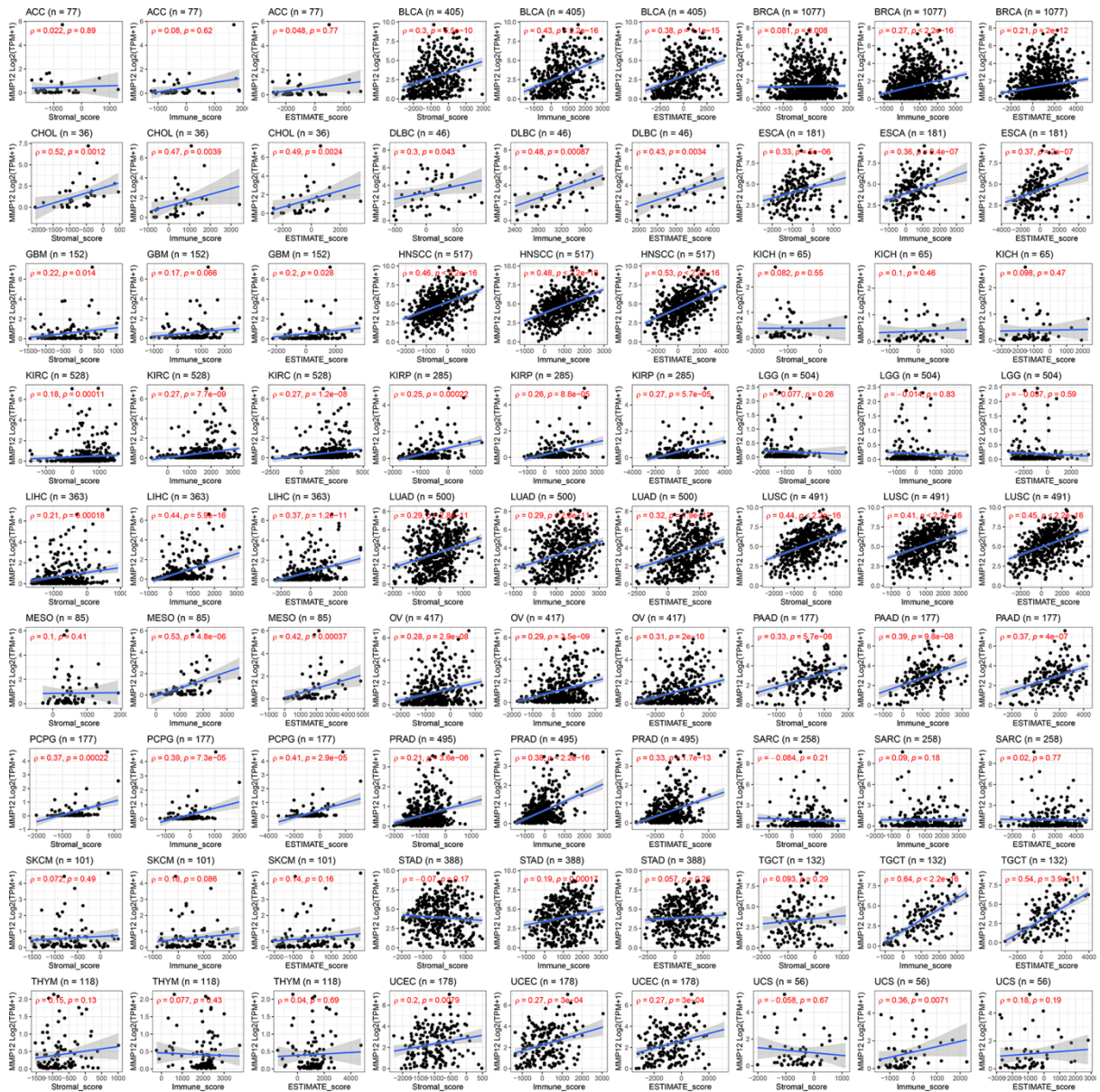
Supplementary material 5. Relationship between MMP12 expression and the ESTIMATE algorithm in multiple cancers.
