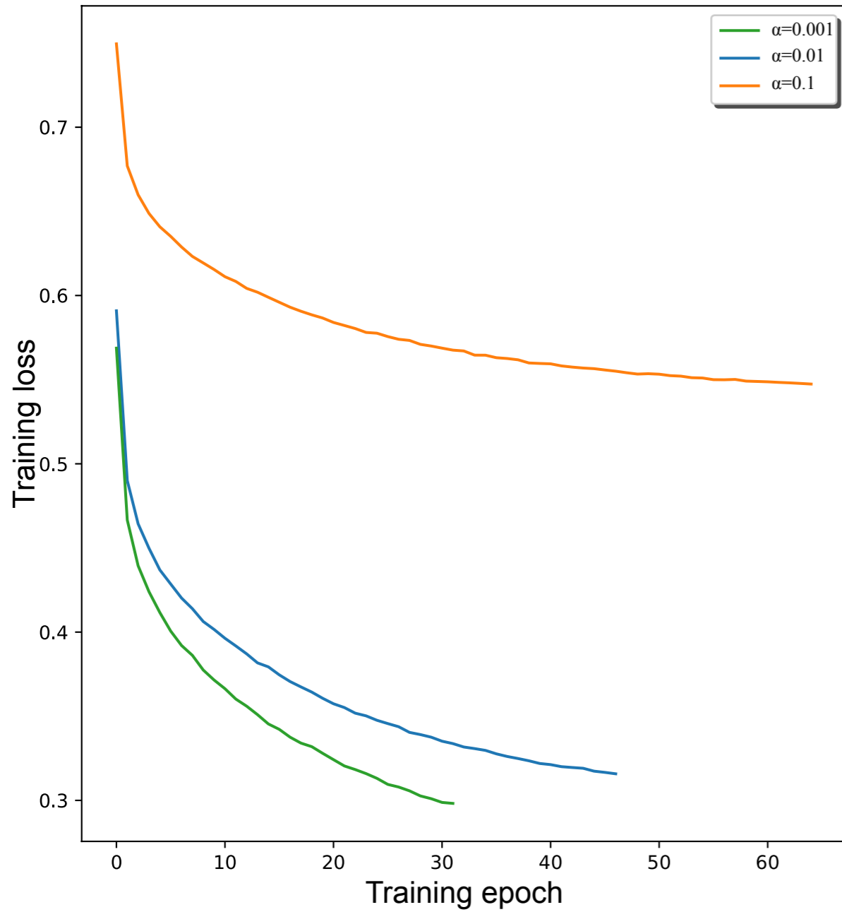
Training/validation loss vs. strength of label smoothing
