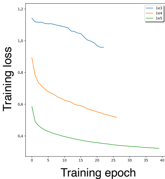
Loss vs. alignment size
