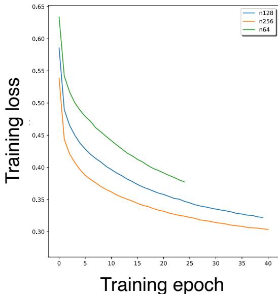
Loss vs. alignment size
