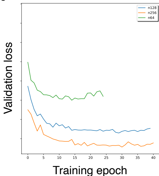
Loss vs. alignment size
