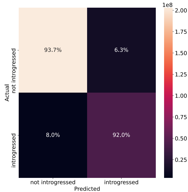
Beneficial: s = 1e-6
