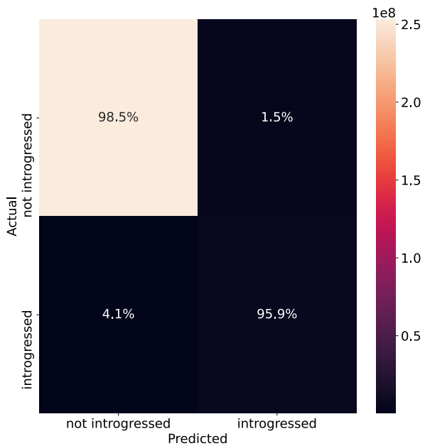
Deleterious: s = -1e-5
