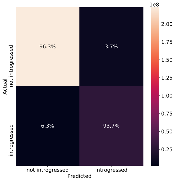
Deleterious: s = -1e-6
