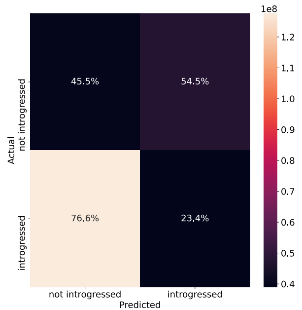
Beneficial: s = 1e-5
