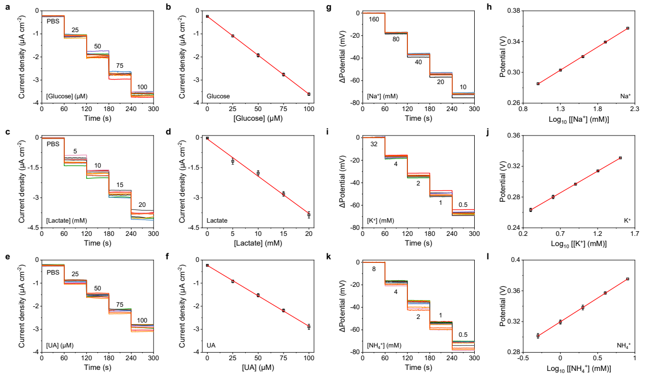
Supplementary Fig. 18 | Reproducibility of biochemical sensors in the CARES. a–l, Batch to batch variation of glucose (a,b), lactate (c,d), UA (e,f), \text{Na}^+ (g,h), \text{K}^+ (i,j), and \text{NH}_4^+ (k,l) sensors. Data is presented as mean \pm SD ( n = 10 sensors for each category).
