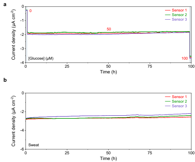
Supplementary Fig. 12 | Long-term stability of continuous 100-hour in vitro tests of wearable glucose biosensors. a,b, Amperometric response of the glucose sensors tested in standard solution (a) and untreated human sweat samples (b) over 100 hours.
