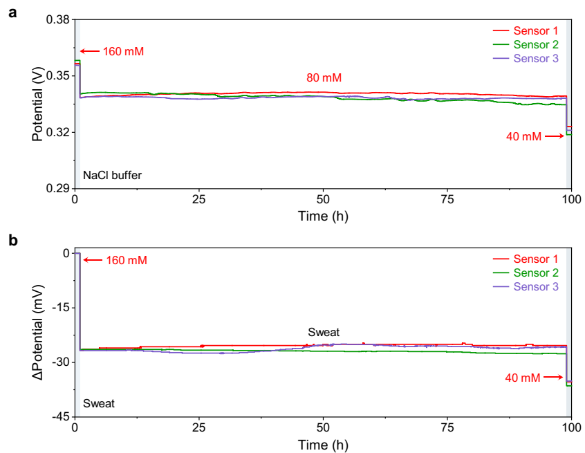
Supplementary Fig. 15 | Long-term stability of continuous 100-hour in vitro tests of wearable ISE-based Na + sensor. a,b , Potentiometric responses of Na + sensors tested in standard solution (a) and untreated human sweat samples (b) over 100 hours.
