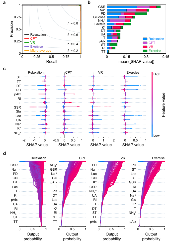
Supplementary Fig. 39 | ML prediction performance of stressor type classification. a, Precision-recall curve of a XGBoost model for each stressor as well as micro-averaged classification result. b, Stacked bar plot of feature importance showing their contribution to each stressor type. c, Shapley additive explanation (SHAP) summary plot with respect to a XGBoost model based on the dataset collected by CARES. d, SHAP decision plot explaining how a XGBoost model arrives at each stressor classification for every data point using both physiological and chemical features. Each decision line tracks the features contributions to every individual classification.
