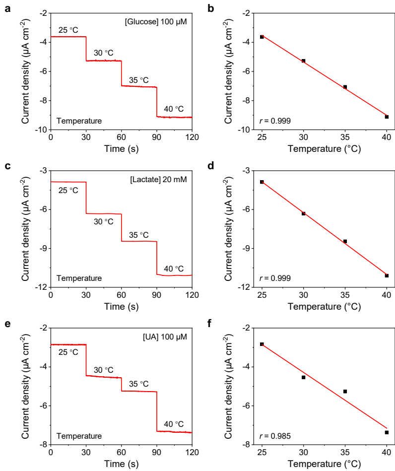
Supplementary Fig. 25 | Temperature influence on enzymatic sensors. a–f, Calibration of glucose (a,b), lactate (c,d), and UA (e,f) biosensors under physiologically relevant range of temperature.
