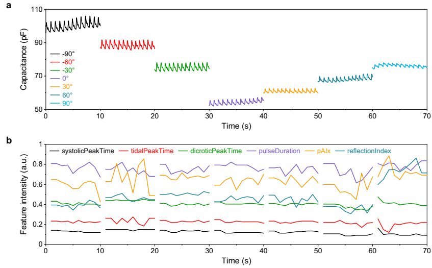
Supplementary Fig. 37 | Pulse signals measured at different wrist angles of a relaxed subject and corresponding extracted features. a , Pulse signal variations when the subject bends the wrist from -90^\circ to 90^\circ , which showed big waveform changes and could cause big variations during daily activities. b , After feature extraction algorithm, the feature remained stable in a moderate angle range from -30^\circ to 30^\circ .
