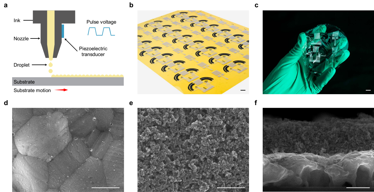
Supplementary Fig. 1 | Characterization of the inkjet-printed CARES electrodes. a , Schematics of inkjet printing mechanism. b , Optical image of a flexible CARES sensor array fabricated via mass-producible and low-cost inkjet printing. Scale bar, 1 cm. c , Optical image of an ultrathin CARES patch on a subject hand. Scale bar, 1 cm. d–f , SEM images of inkjet-printed Ag ( d ), carbon ( e ), and cross-section of Ag-carbon interconnect ( f ). Scale bars, 500 nm.
