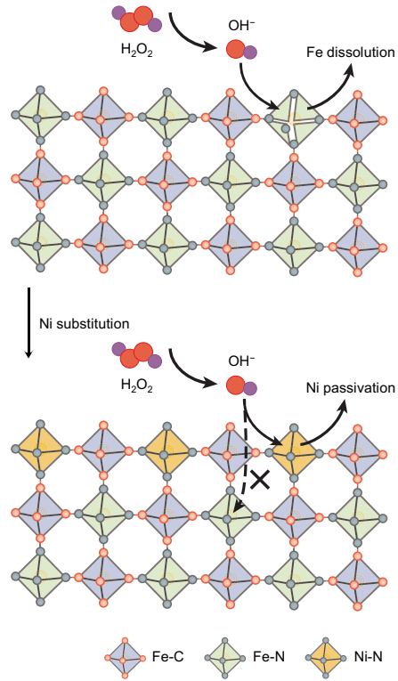
Supplementary Fig. 8 | Schematic of passivation mechanism of PB-NiHCF. Hydroxide ions ( OH^- ) can break Fe-(CN)-Fe bond while nickel serves as protection layer to prevent PB degradation.
