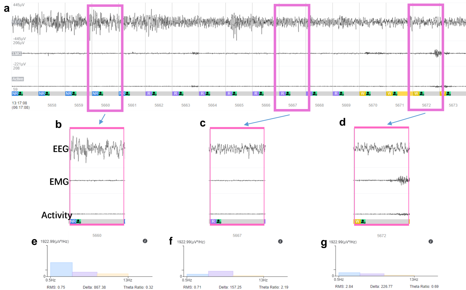
Fig. S5 Real operation window of vigilance scoring. a paradigm of EEG/EMG/Activity raw data in a 80-s recording period. b-d Typical examples of SWS (labeled as NR), REM sleep (labeled as R) and wakefulness (labeled as W) in a 4-s epoch counting unit, respectively. e-g Typical examples of FFT of SWS (matching with b ), REM sleep (matching with c ) and wakefulness (matching with d ) in a 4-s epoch counting unit, respectively.
