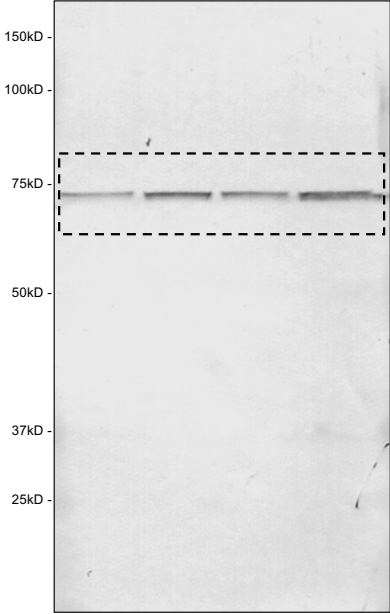
eIF3D
