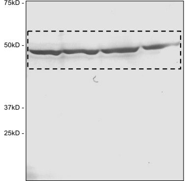
Actin
