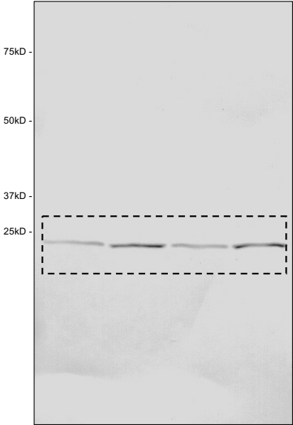
COX4
