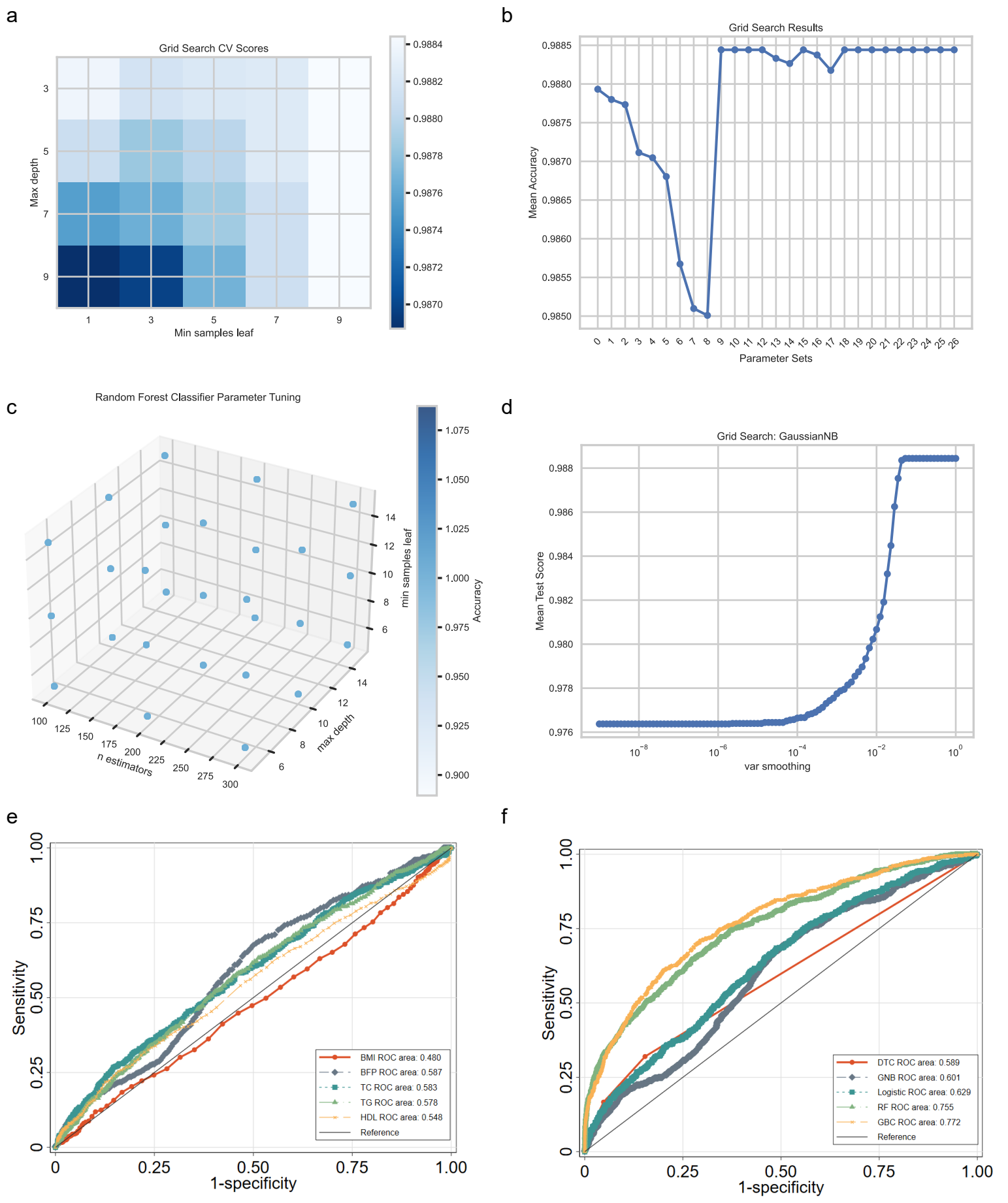
Supplementary figure 1: Tuning process for different machine learning models. (a) Decision Tree Classifier model; (b) Gradient Boosting Classifier model; (c) Random Forest Classifier model; (d) GaussianNB model; (e) ROC Curves of Different Obesity Indicators Individually Predicting RIS; (f) Roc curves for RIS prediction by different machine learning models
