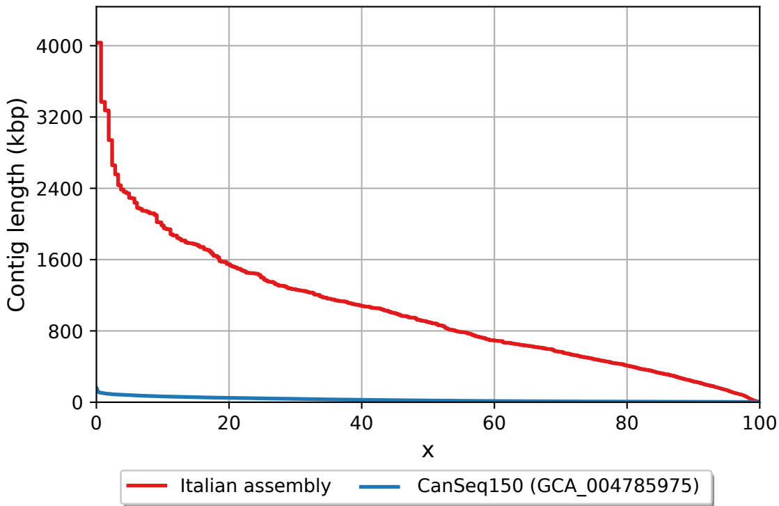
Supplementary Figure 2. QUAST-LG Nx comparison between the Italian genome and the CanSeq150 Canadian genome. The contiguity of the new Italian assembly is extremely higher than the CanSeq150 genome.
