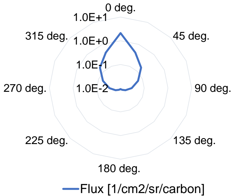
Supplemental Fig.1 The angular distribution of neutrons evaluated via PHITS calculations.
