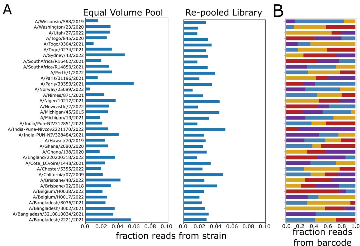
Figure S2. Sequencing-based pooling of library to try to achieve equal transcriptional titers across viruses. A) We first infected cells with equal volumes of the stocks of the viruses with each of the 36 different HAs in the library, and then sequenced the viral barcodes to quantify the fraction of barcodes attributable to each virus, as plotted at left. We then re-pooled the virus stocks to try to achieve equal barcode representation for each virus stock. The plot at right shows the fraction of barcodes attributed to each virus after the re-pooling. This re-pooled mix was used in all experiments in this study. C) The fraction of barcode reads attributable to each of the two to four unique barcodes for each virus in the re-pooled libraries. Each row represents a different virus strain and each color represents a different barcode, with the width of each stacked bar representing the fraction of counts for that strain that are attributable to each of the two to four barcodes for the strain.
