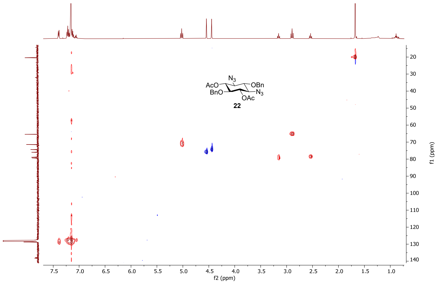
HSQC NMR Spectra (500 MHz, Benzene- d_6 ) of 4,6-Di-O-acetyl-1,3-di(deamino)-1,3-diazido-2,5-di-O-benzylstreptamine ( 22 )
