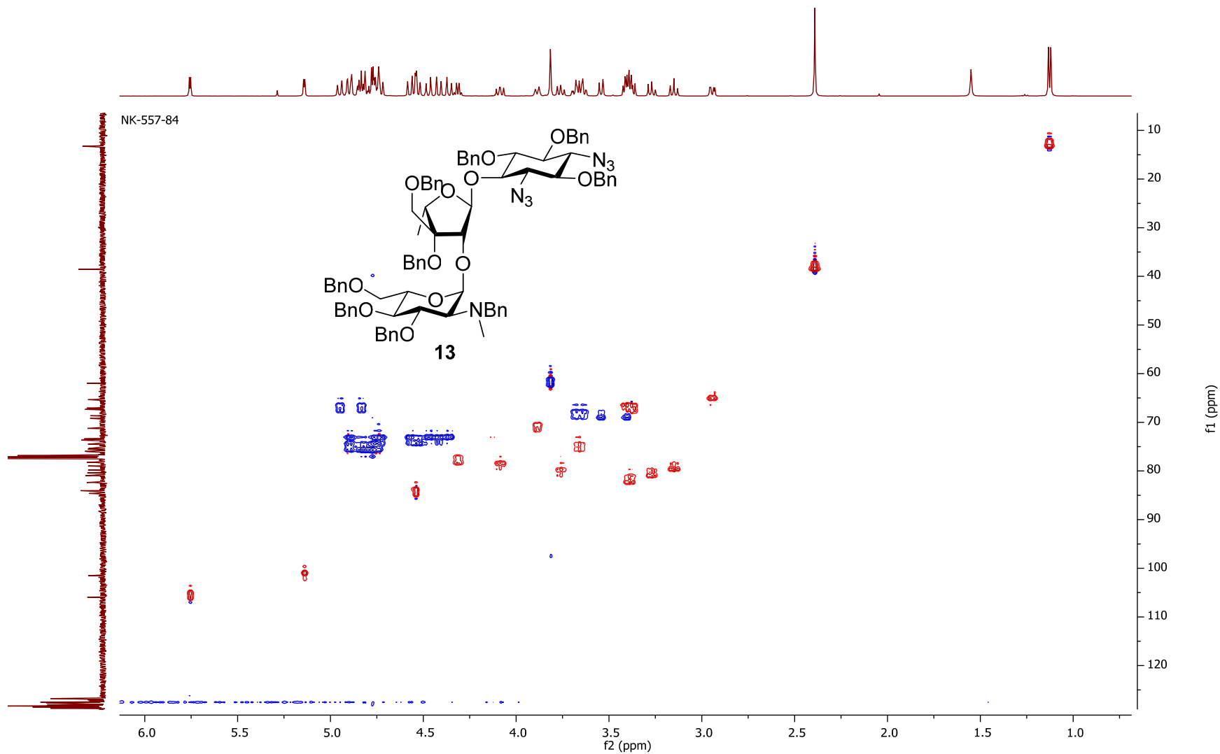
HSQC NMR (500 MHz, CDCl 3 ) spectrum of 1,3-bis(deamino)-1,3-diazido-2,5,6-tri-O-benzyl-4-O-(3',6'-di-O-benzyl-2'-O-(2''-N-benzyl-3'',4'',6''-tri-O-benzyl-dihydrostreptomycin (13)
