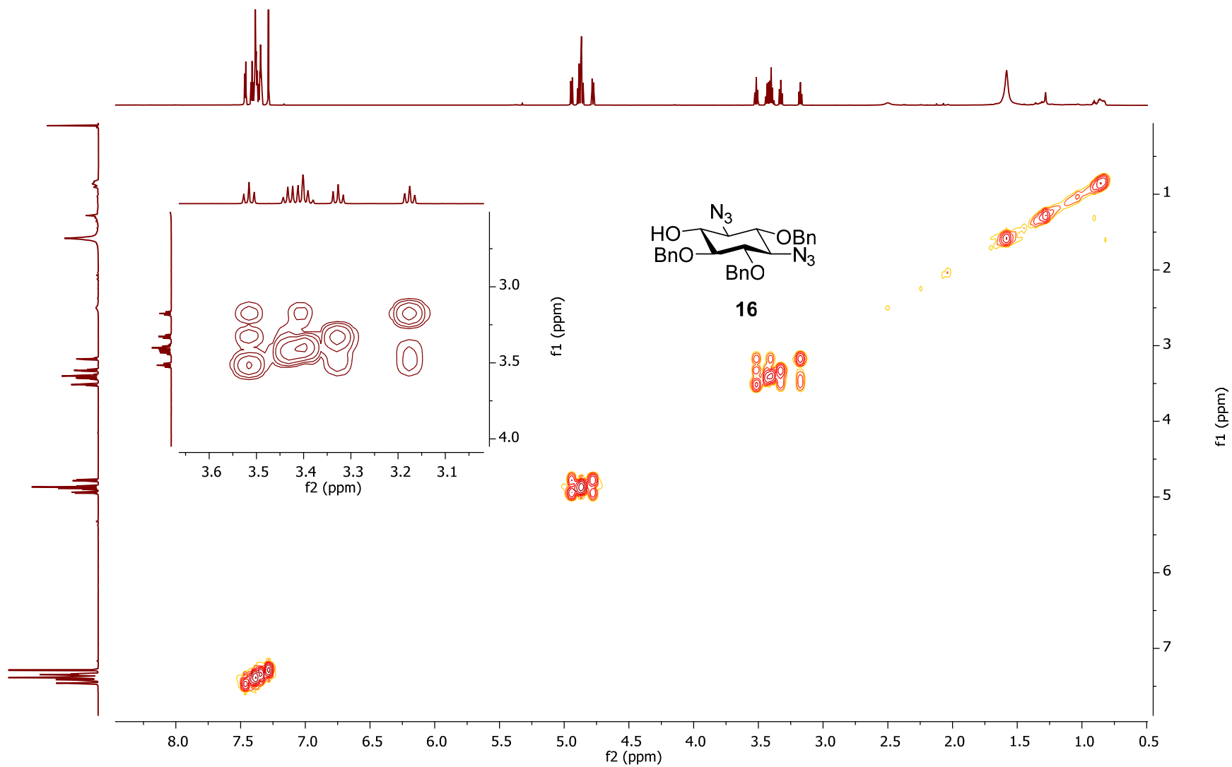
COSY NMR (900 MHz, CDCl 3 ) spectrum of 1,3-Di(deamino)-1,3-diazido-2,5,6-tri-O-benzyl streptamine ( 16 )
