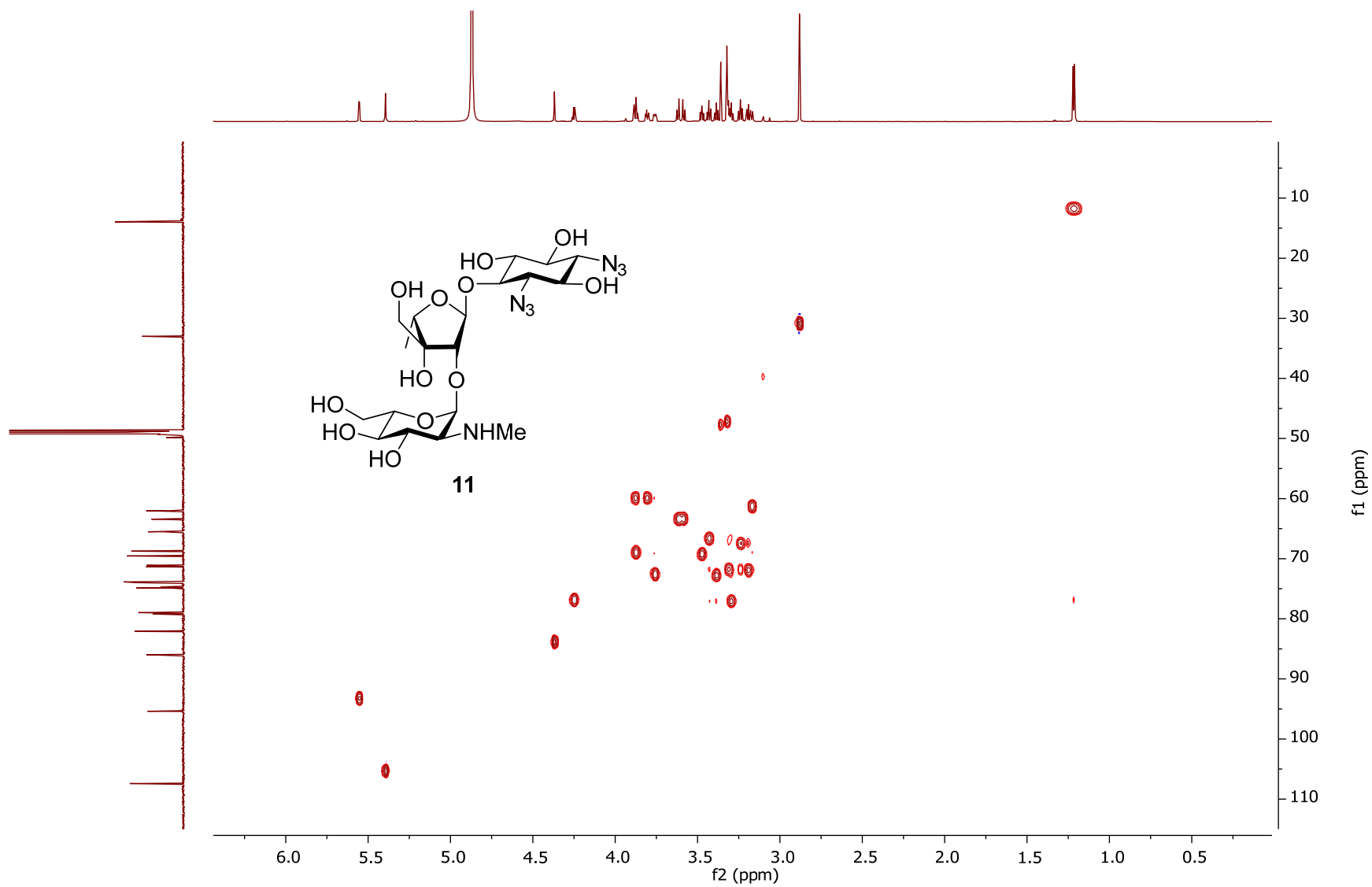
HSQC NMR (900 MHz, CD 3 OD) spectrum of 1,3-bis(deamino)-1,3-diazido-dihydrostreptomycin ( 11 )
