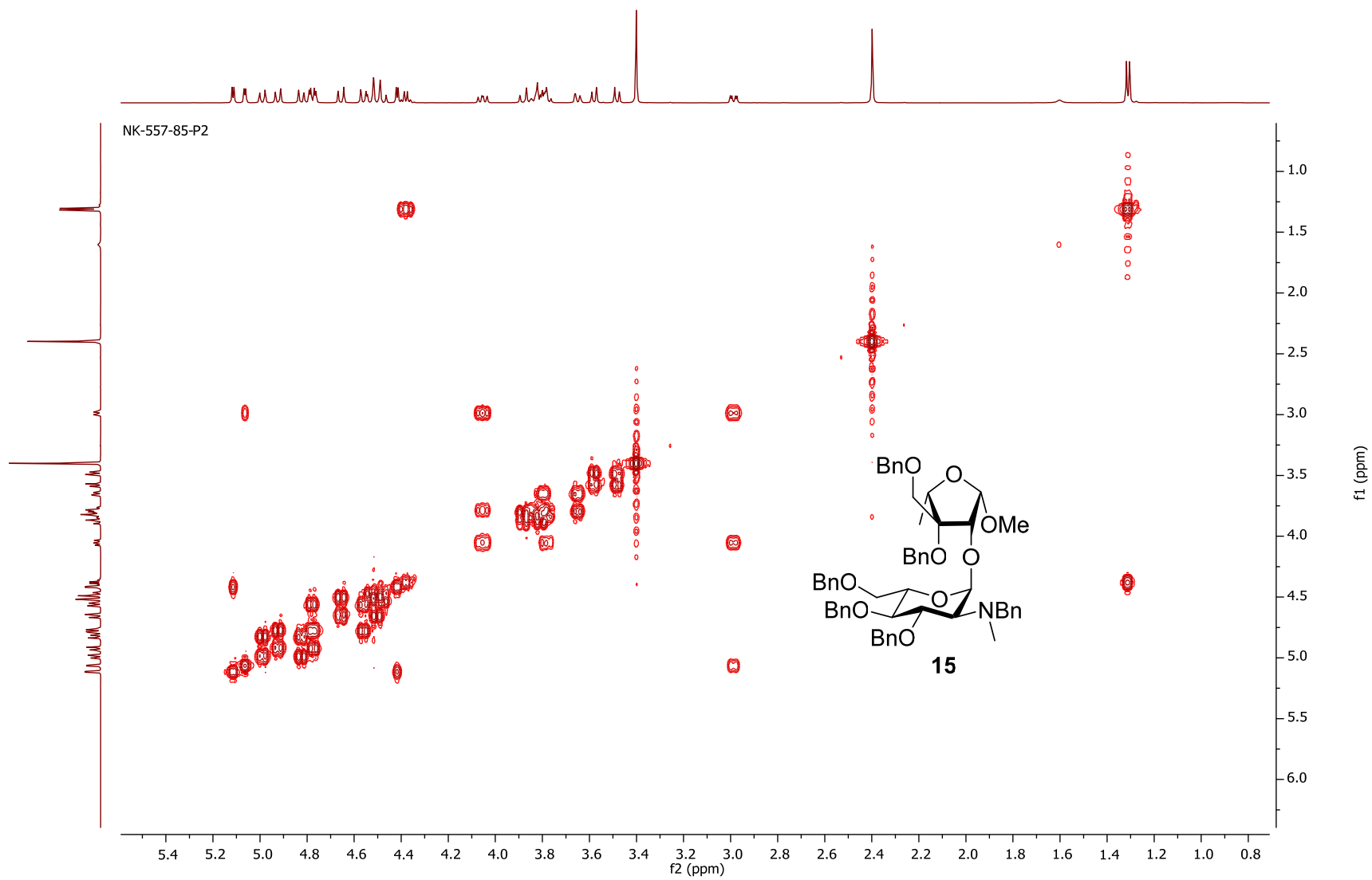
COSY NMR (500 MHz, CDCl 3 ) spectrum of Methyl 3',6'-di-O-benzyl-2-O-(2''-N-benzyl-3'',4'',6''-tri-O-benzyl)-β-streptobiosaminide (15)
