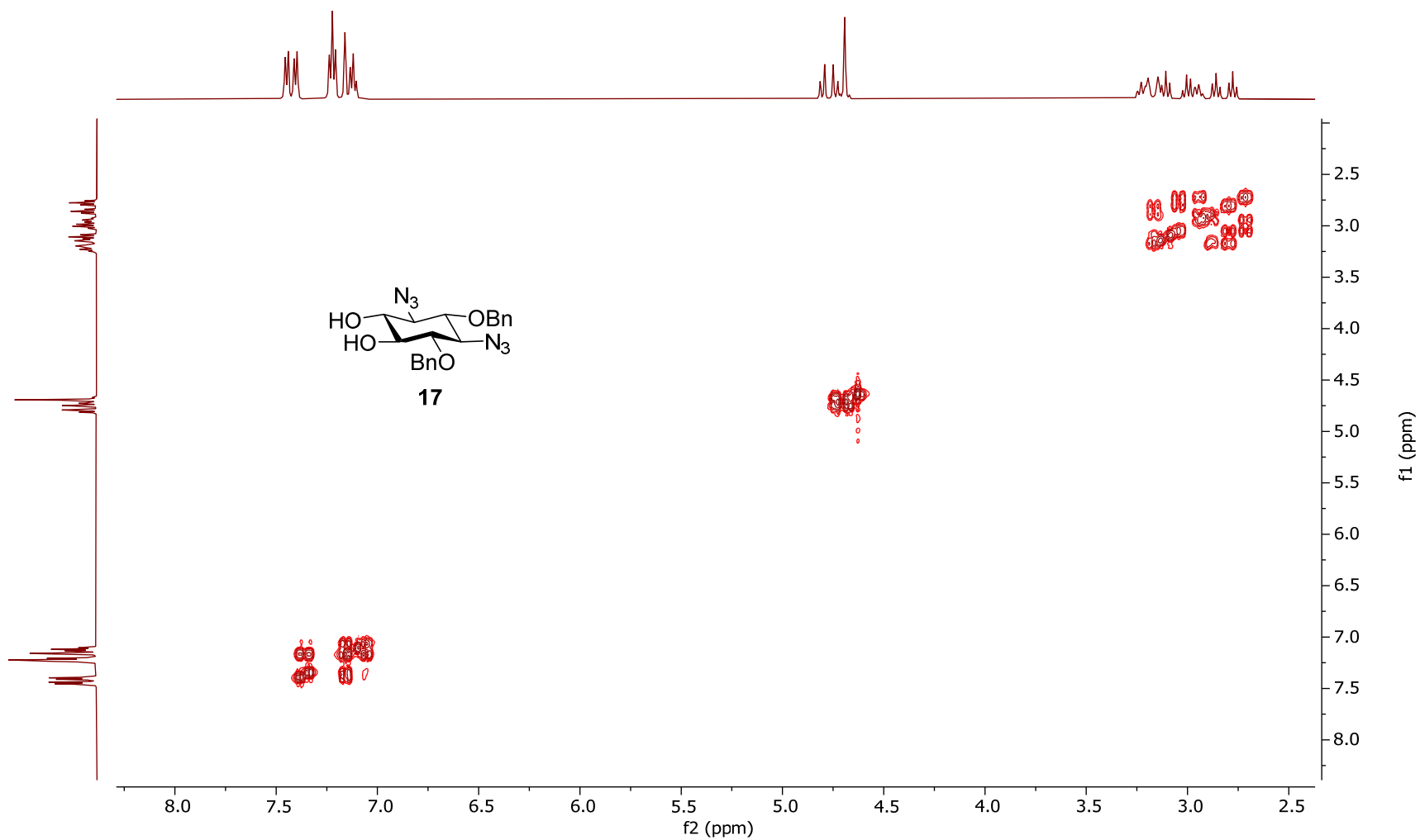
^1\text{H} - ^1\text{H} COSY NMR Spectra (500 MHz, Benzene- d_6 ) of 1,3-Di(deamino)-1,3-diazido-2,6-di-O-benzylstreptamine ( 17 )
