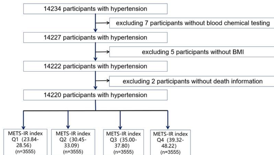
Figure S1: Research population selection process diagram.
