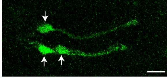
S3 Fig. Ir21a-QF2w labels three neurons in each DOG. Genotype: Ir21a-QF2w/QUAS-GCaMP3 . White arrow: cell body. Scale bar: 10 \mu m.
