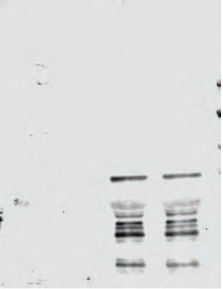
Methyalmalonylation
