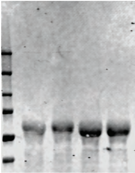
Acetylation
