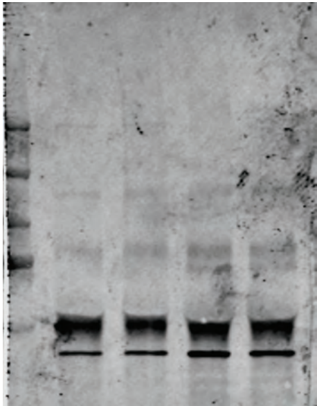
Succinylation
