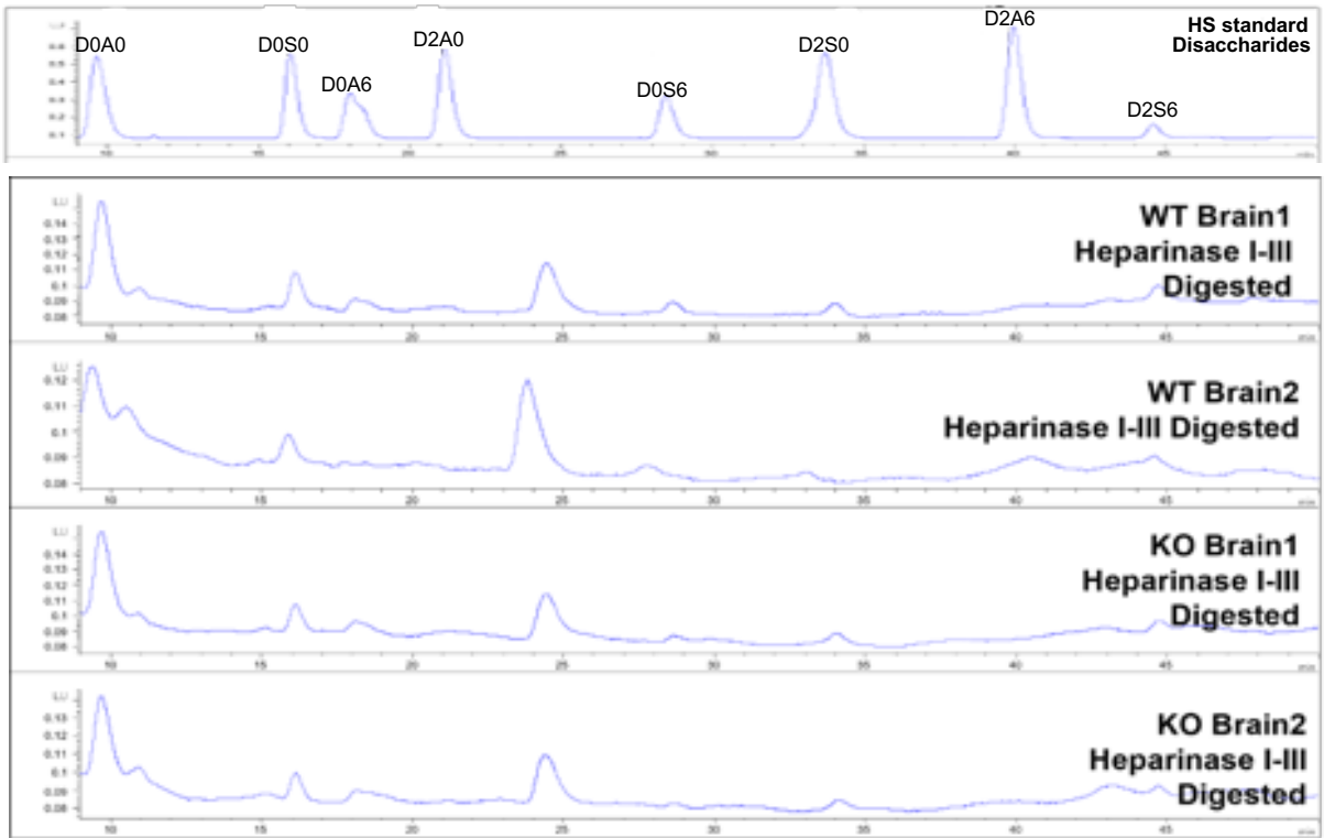
Supplementary Figure S3. SAX-HPLC. (A) Diagram showing the SAX-HPLC process. (B) SAX-HPLC chromatographs.
