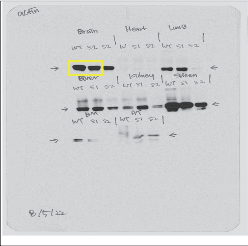
Brain_β-actin
