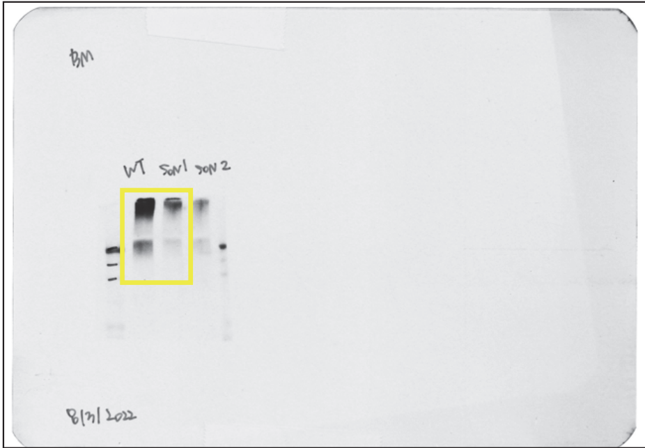
Bone marrow_Son
