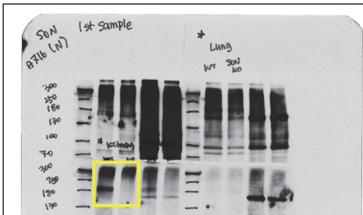
Kidney_Son
