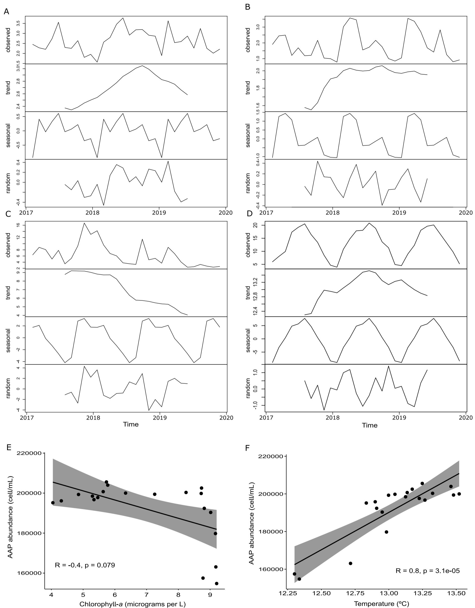
Supplementary Figure S7 : Decomposition of additive time series for bacterial abundance (A), AAP abundance (B), chlorophyll - a concentration (C) and temperature (D). Analysis was done in the TTR package version 0.24.3 (R version 4.3.0). Spearman correlation of the decomposed trends between AAP abundance and chlorophyll- a (E) and AAP abundance and temperature (F). R: spearman's rho value, p: p-value.
