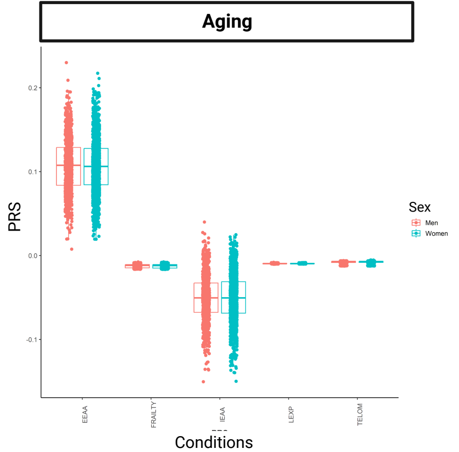
Supplementary Figure S4. Distribution of Polygenic Risk Scores by sex. Adjusted FDR p-values are reported.
