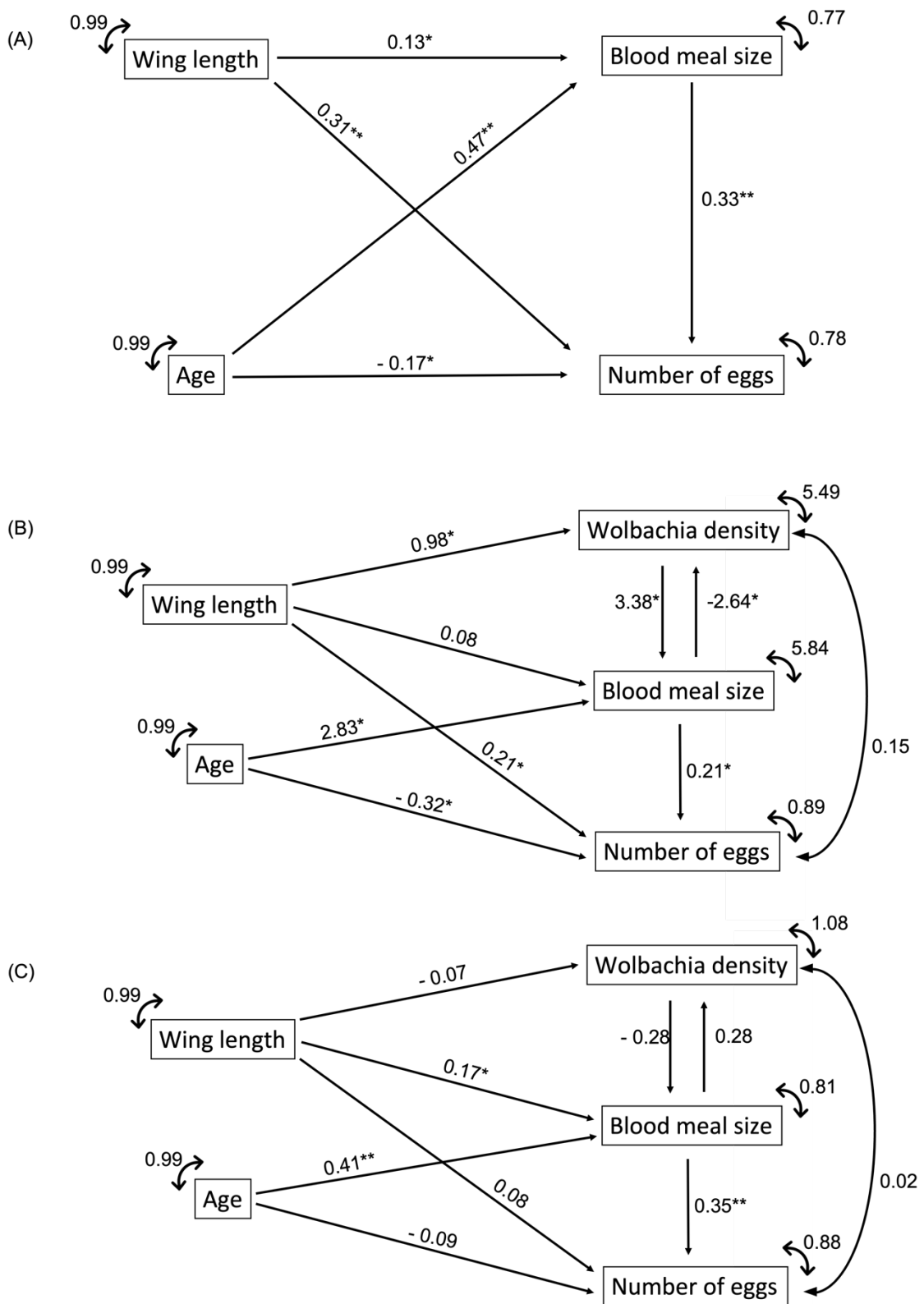
Supplementary Figure 2: Full model path diagrams for: (A) Wolbachia -uninfected field population, (B) wMel , and (C) wAlbB . Numbers over the arrows are the path coefficients and their statistical significance is indicated as follows: * P < 0.05 , ** P < 0.01 .
