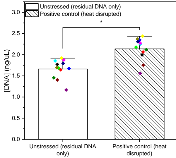
Figure S1 - Free residual DNA in unstressed viral stock vs. total DNA in heat disrupted sample. Increase in DNA is statistically significant ( p -value < 1E-06 ). Colored symbols denote measurements from the same experiment. Data points are offset for visual clarity. The top line of each box represents the mean value of the dataset, and the error bar represents the data range within 1.5 times the interquartile range.
