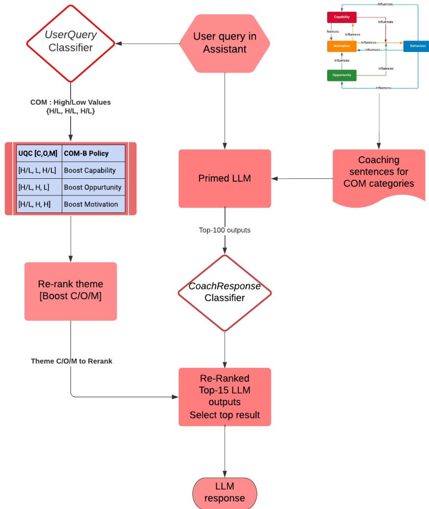
S2 Fig: Priming and BeSci infusion to LLM framework pipeline in Fit-LLM for user query input
