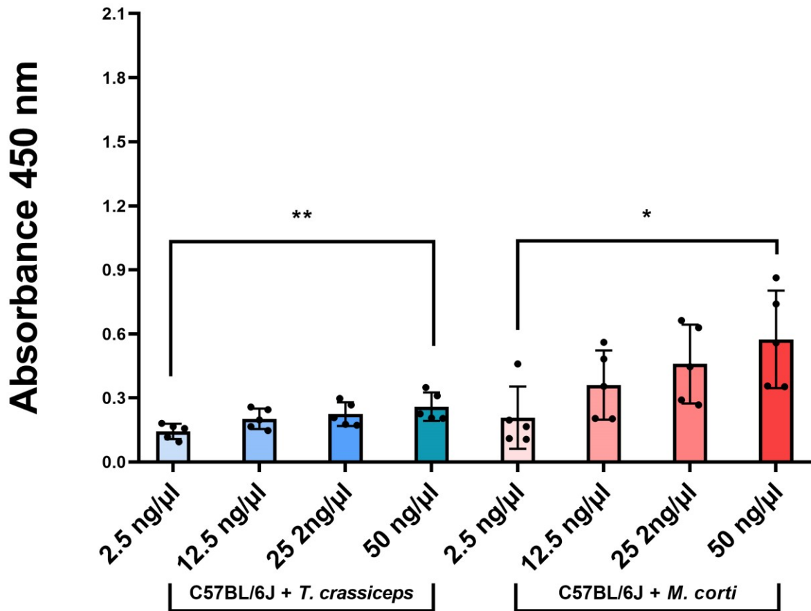
SFig. 4. Titration of MelH antigen. There was significant change in IgM binding to MelH only when the antigen concentration was increased 20x, showing that the IgM probably bound to the antigen only in a non-specific manner, after analysis with Kruskal-Willis test with Dunn's multiple comparisons. C57BL/6J mouse sera were tested (n = 5), infected with either T. crassiceps or M. corti .
