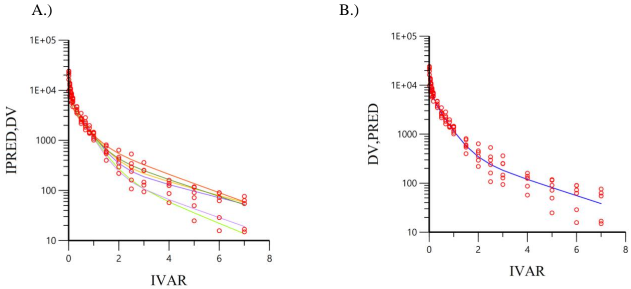
Supplementary Figure 1. (A) Plot of dependent variable (DV; concentrations) and individual prediction (IPRED) vs independent variable (IVAR; time) (B) Plot of dependent variable (DV; concentrations) and population prediction (PRED) vs the independent variable (IVAR: time).
