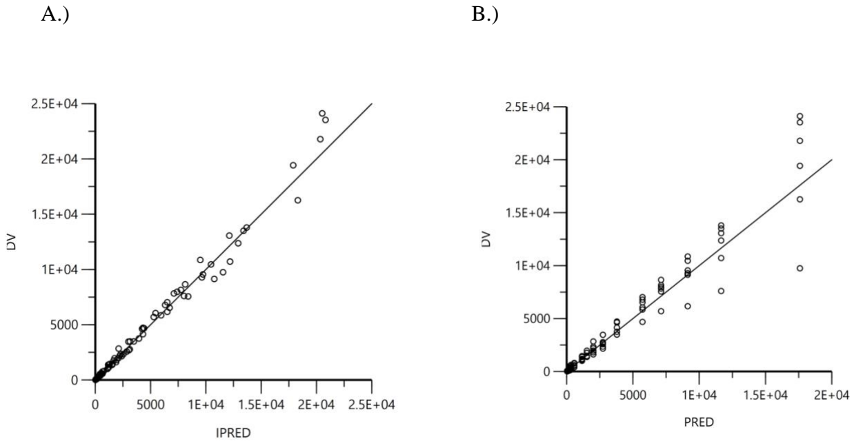
Supplementary Figure 2. (A) Plot of the dependent variable (DV; concentrations) versus individual predicted values (IPRED; predicted concentrations) and (B) Plot of the dependent variable (DV; concentrations) versus population predictions (PRED)
