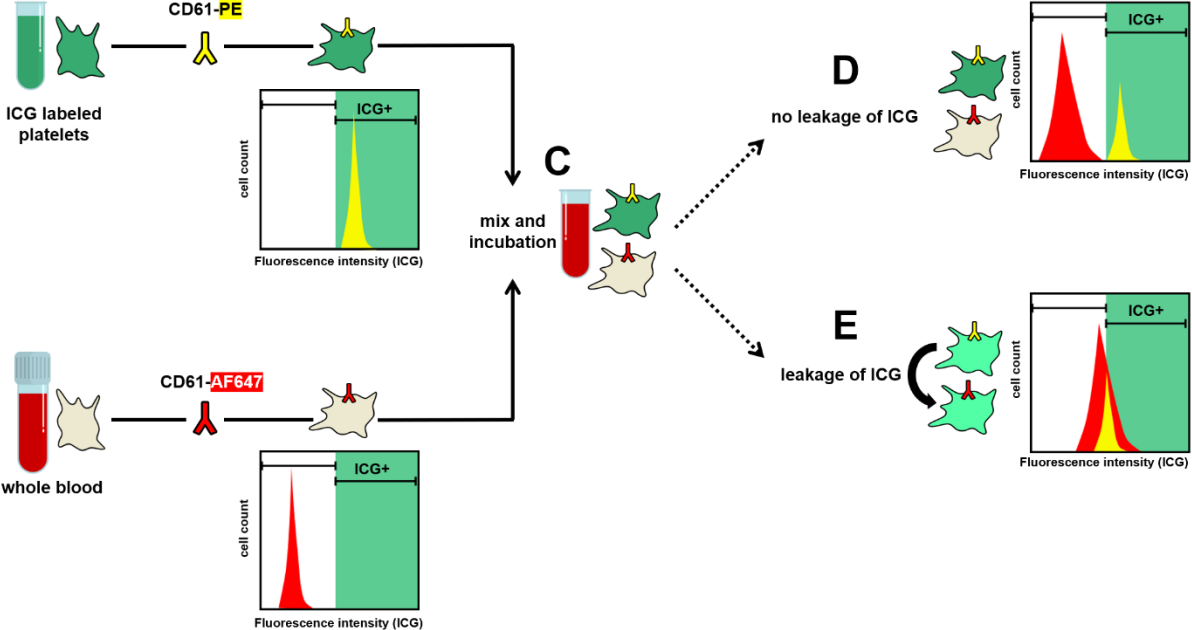
Figure S1. Flow cytometric analysis after addition of whole blood to ICG-labeled platelets (10 μM ICG final concentration in 100% PAS-E). In 100% PAS-E leakage of ICG from labeled platelets was not observed resulting in sufficient differentiation between labeled platelets from platelet concentrates and non-labeled platelets from whole blood. Labeling platelets in plasma containing additive solution leakage generated insufficient labeling with subsequent leakage of ICG from labeled platelets.
