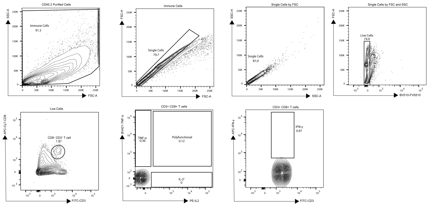
Supplementary figure 10. Gating strategy for analyzing intracellular cytokine (ICS) staining of CD8 + T cells isolated from MC-38 tumours. Within CD8 + T cells, defined CD3 + CD8 + , expression of the cytokines IFN- \gamma , TNF- \alpha , and IL-2 was analyzed.
