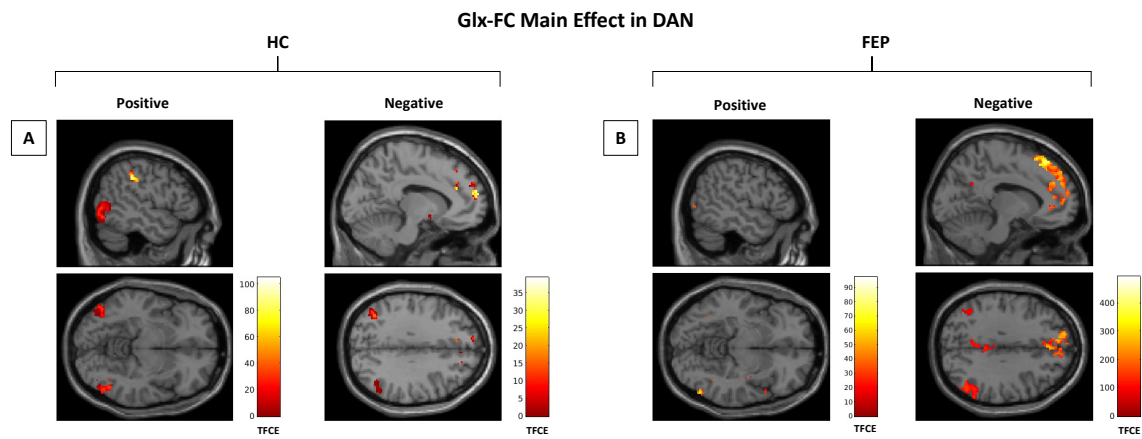
Supplementary figure 2. Clusters indicate correlations between positive/negative FC and Glx in A) HC and B) FEP in the DAN (TFCE corrected). DAN, dorsal attention network; TFCE, threshold-free cluster enhancement; HC, healthy controls; FEP, first episode psychosis.
