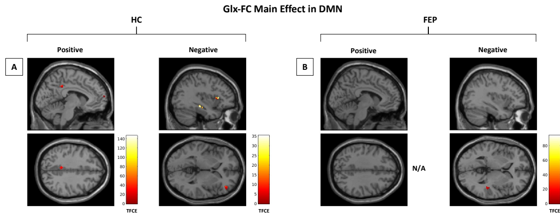
Supplementary figure 1. Clusters indicate correlations between positive/negative FC and Glx in A) HC and B) FEP in the DMN (TFCE corrected). DMN, default mode network; TFCE, threshold-free cluster enhancement; HC, healthy controls; FEP, first episode psychosis.
