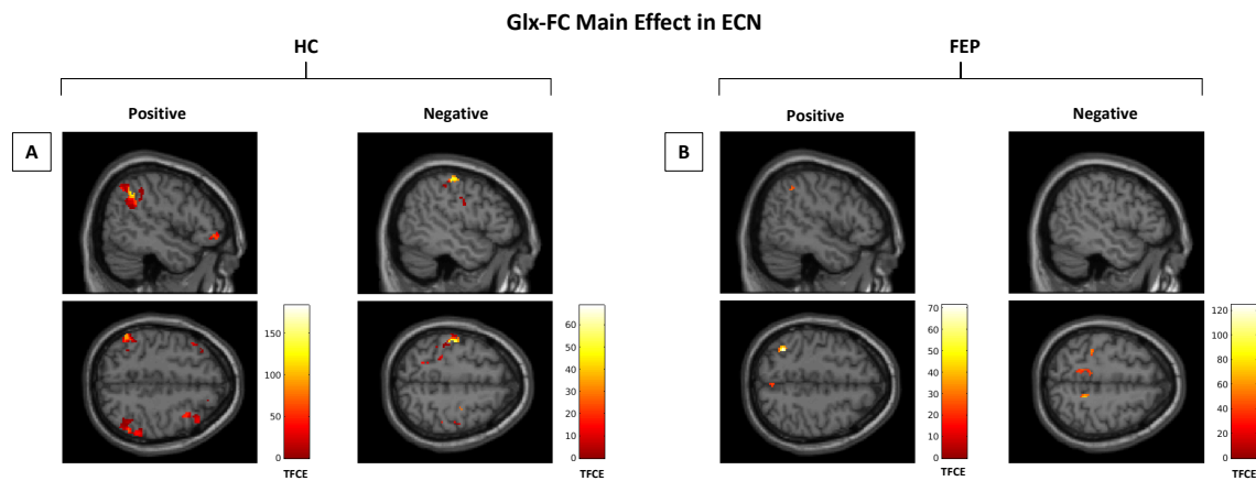
Supplementary figure 3. Clusters indicate correlations between positive/negative FC and Glx in A) HC and B) FEP in the ECN (TFCE corrected). ECN, executive control network; TFCE, threshold-free cluster enhancement; HC, healthy controls; FEP, first episode psychosis.
