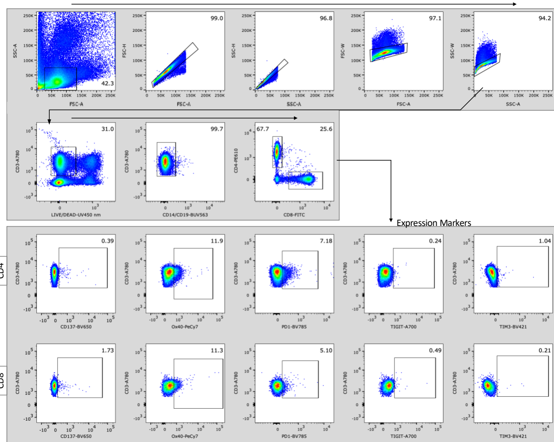
Supplemental Digital Content 4. Gating strategy for Activation/Exhaustion panel. Approach for identifying T cells expressing various activation or exhaustion markers.
