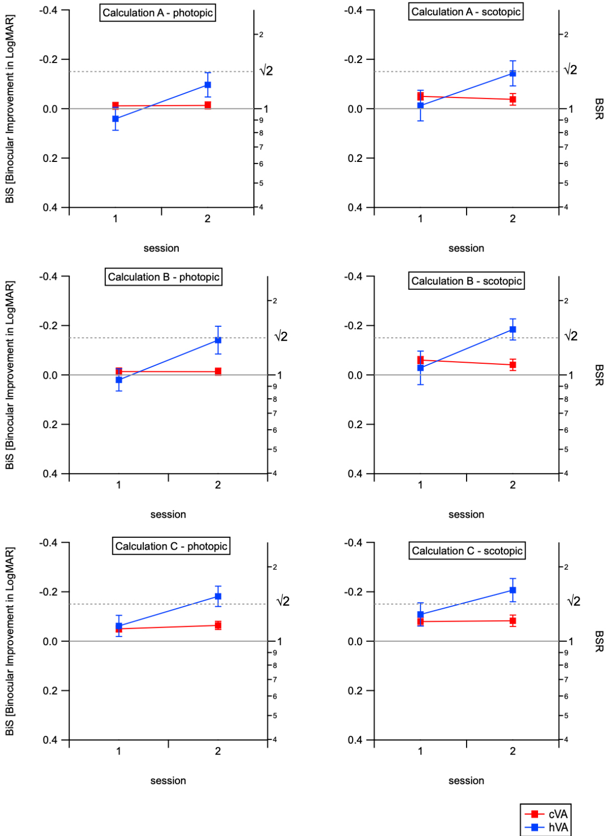
Figure 2 supplementary. BiS comparison between sessions. For each of the three approaches (Calculation A-C) BiS is shown for both luminance conditions as binocular improvement (BiS) in logMAR and BSR. Group average and SEM are displayed for cVA and hVA on both days.
