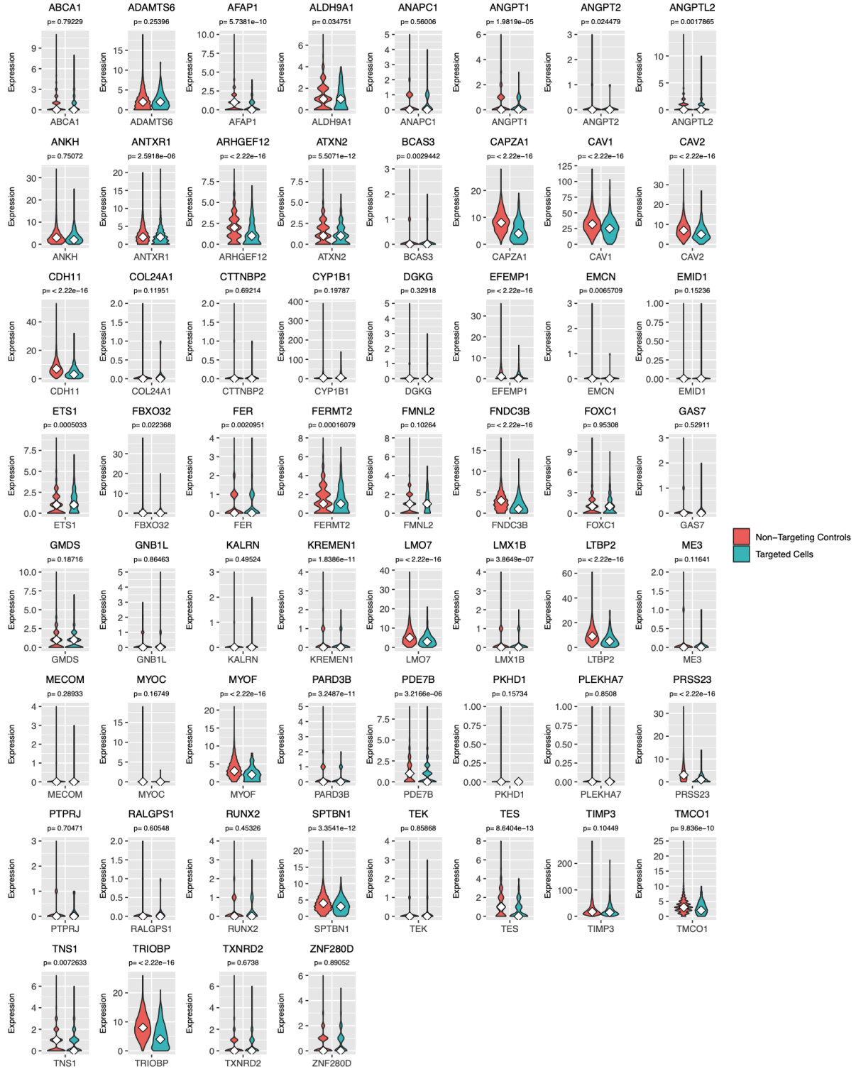
Supplementary Figure 2: Comparison of gene expression levels between each target knockout cell line and non-targeting control cells. ABO and TEX41 were found not to be expressed in our TMCs. P-values are displayed from the Student t-test.
