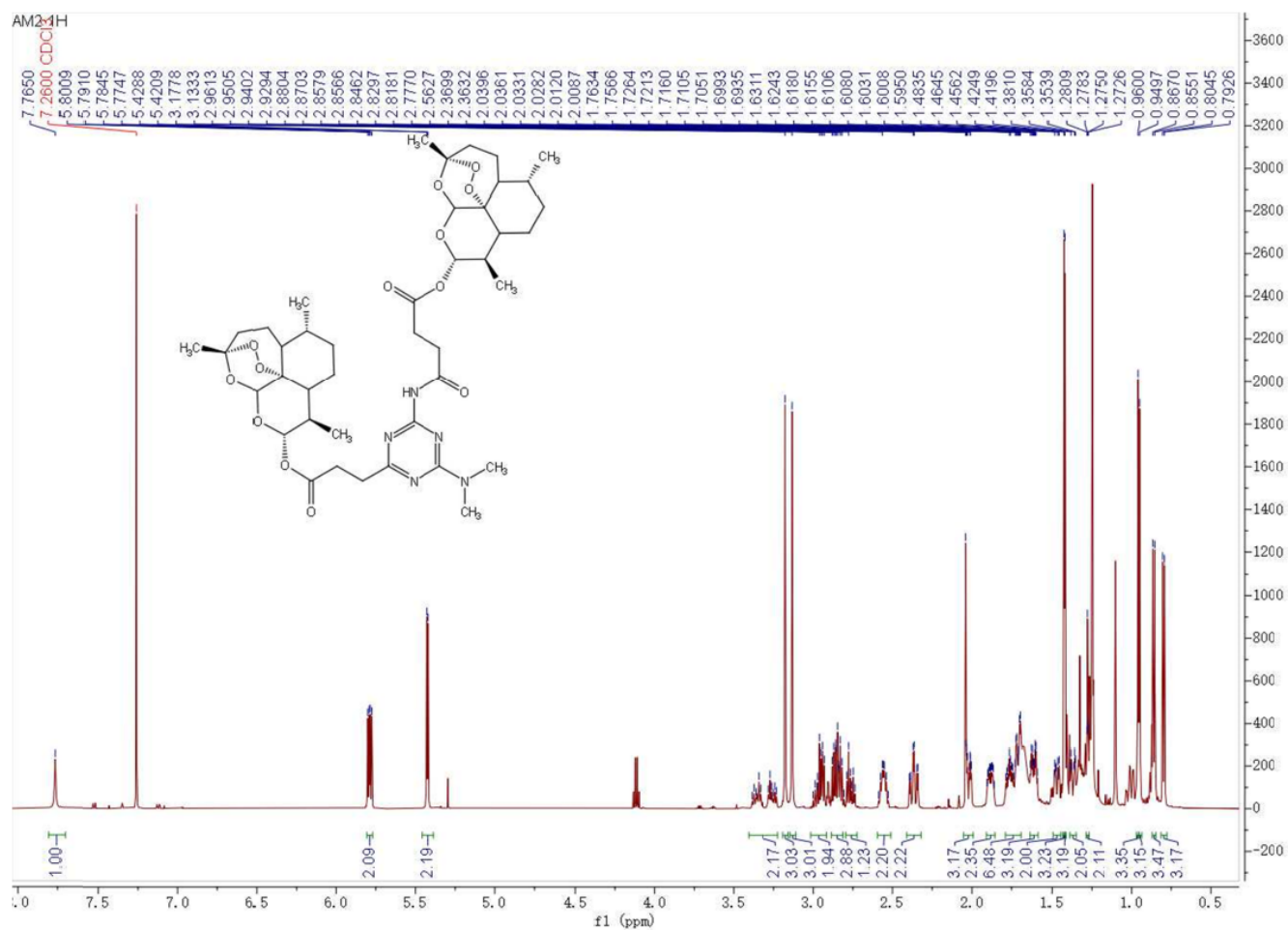
Supplementary Fig. 1. 1 H NMR spectrum of AM2.
