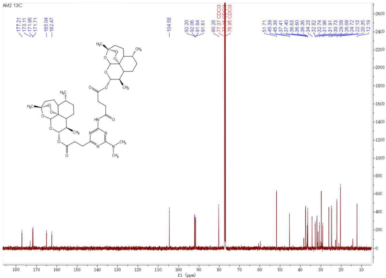
Supplementary Fig. 2. 13 C NMR spectrum of AM2.
