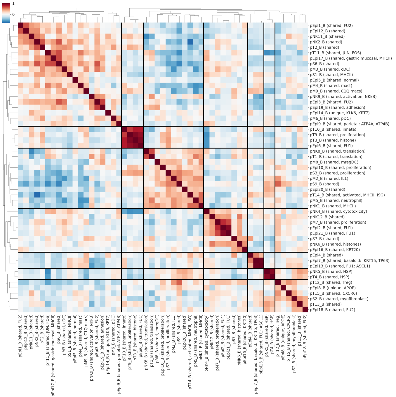
Figure S15. Heatmap showing pairwise correlation of gene program activities across all patient samples at baseline using the 90th percentile of patient-level program activity in epithelial, myeloid, T, NK and stromal cells. Hierarchical clustering was performed to identify clusters of co-varying proteins.
