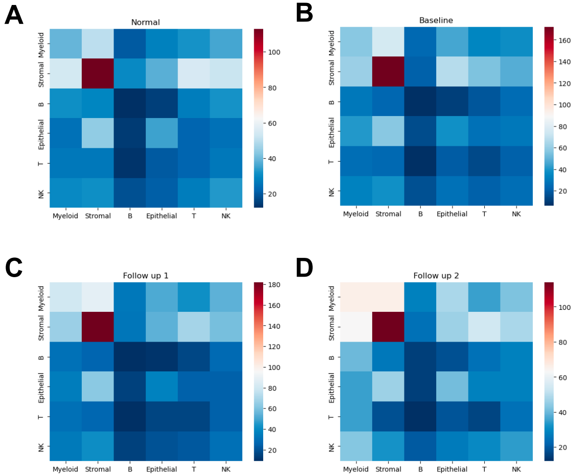
Figure S23. Heatmaps showing the number of significant inferred ligand-receptor interactions between major cell types using CellPhoneDB on scRNAseq data in (A) normal, (B) baseline tumor, (C) post-chemotherapy (FU1) tumor and (D) post-immunotherapy (FU2) tumor samples.
