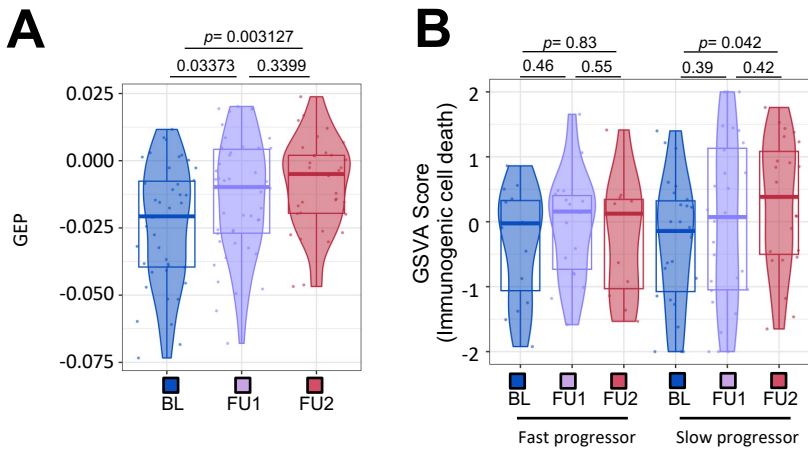
Figure S24. (A) Immune gene expression program signature scored from bulk RNA-seq profiles across all samples separated by timepoint. (B) Immunogenic cell death signatures scored from bulk RNA-seq profiles split by fast and slow progressing patients and by timepoint.
