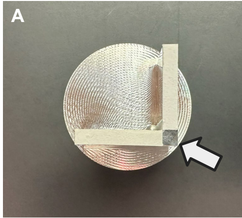
Figure S4: Stamping Procedure. A. Dried bacteriophage and antibiotic strips are aligned at 90° using the right-angle edge of the stamp column. The square region marked by arrow indicates that strips are not overlapping and aligned at 90°. B. The solidified plate is inverted and gently stamped onto the aligned strips. C. Top view of the stamping process. L-shape should be stamped so that there is plenty of room for bacteriophage and antibiotic strips to demonstrate proper clearing.
