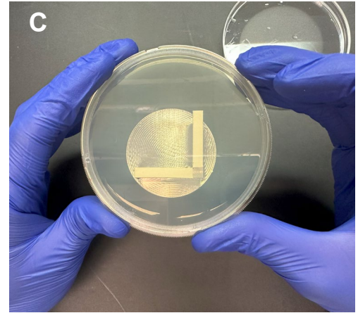
Figure S4: Stamping Procedure. A. Dried bacteriophage and antibiotic strips are aligned at 90° using the right-angle edge of the stamp column. The square region marked by arrow indicates that strips are not overlapping and aligned at 90°. B. The solidified plate is inverted and gently stamped onto the aligned strips. C. Top view of the stamping process. L-shape should be stamped so that there is plenty of room for bacteriophage and antibiotic strips to demonstrate proper clearing.
