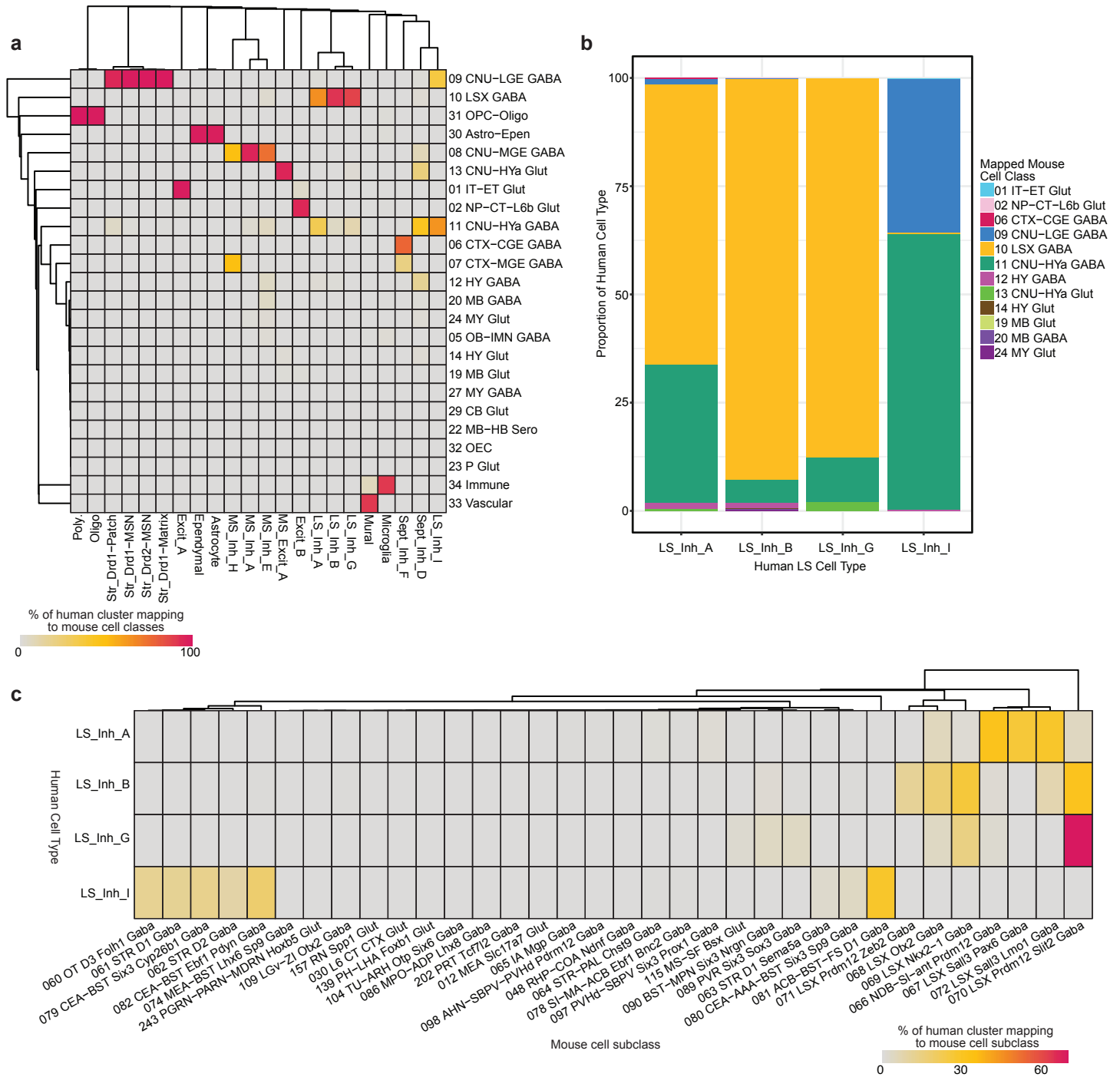
Figure S4. Cross-species analysis with MapMyCells. a , Heatmap of the percentage of each human cell cluster mapping to broad mouse cell classes. b , Barplot for the proportion of each human LS neuronal cell type mapping to broad mouse cell classes. c , Heatmap of the percentage of each human LS neuronal cell type mapping to mouse subclasses.
