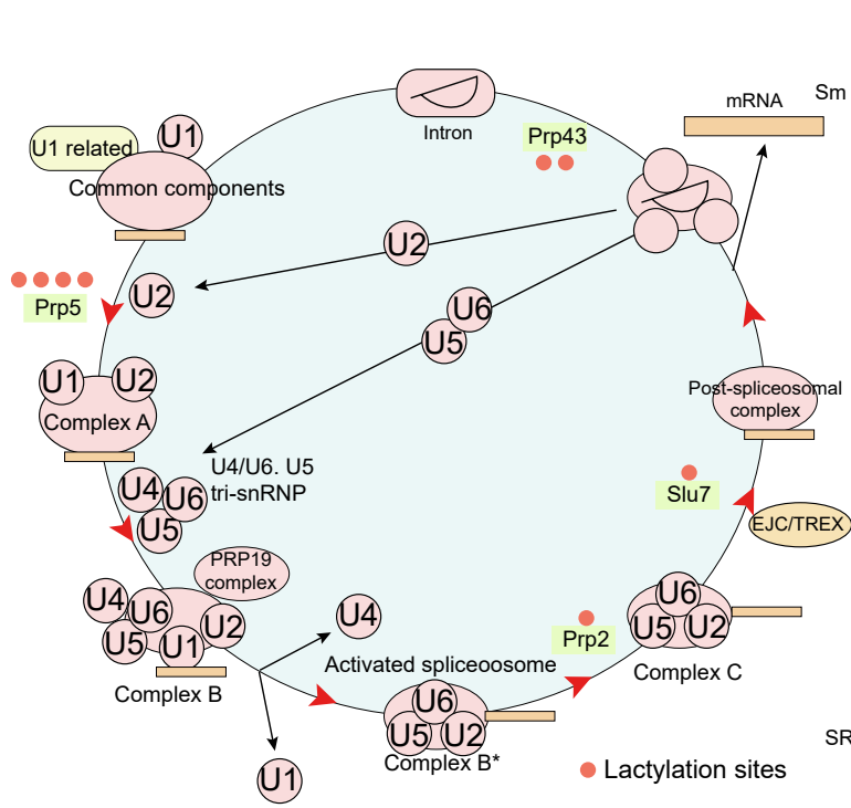
Spliceosome
