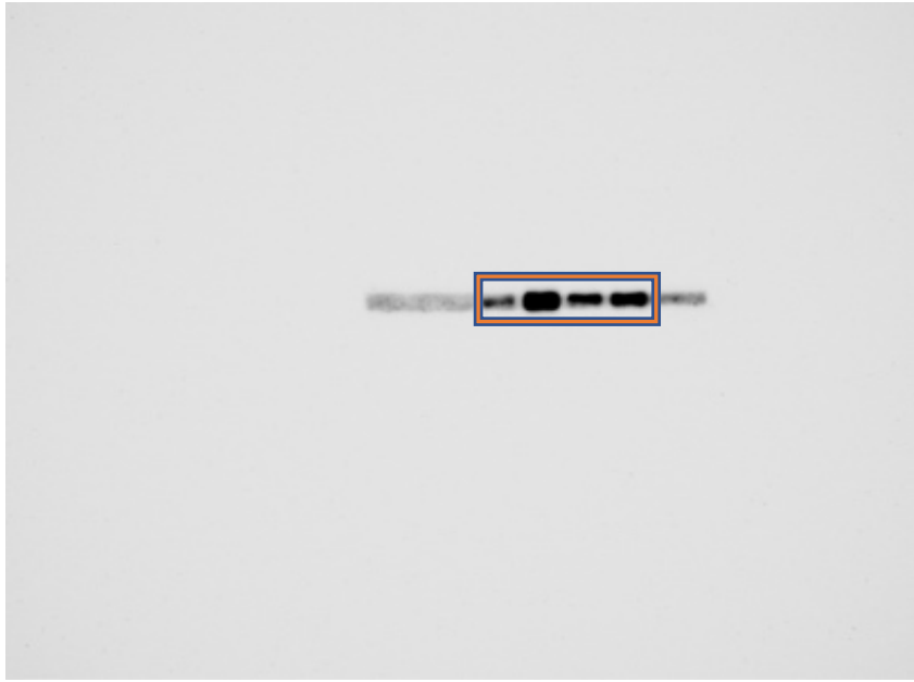
P65/NF-kB
