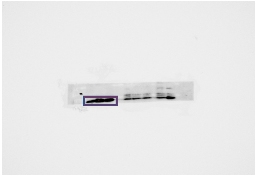
LC3B
