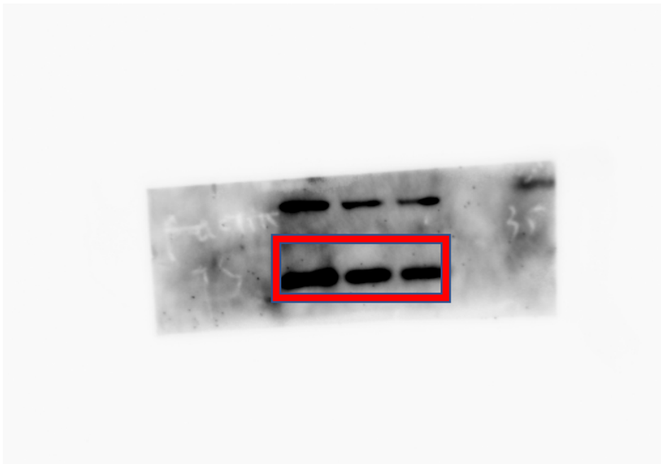
Figure4 \beta -actin
