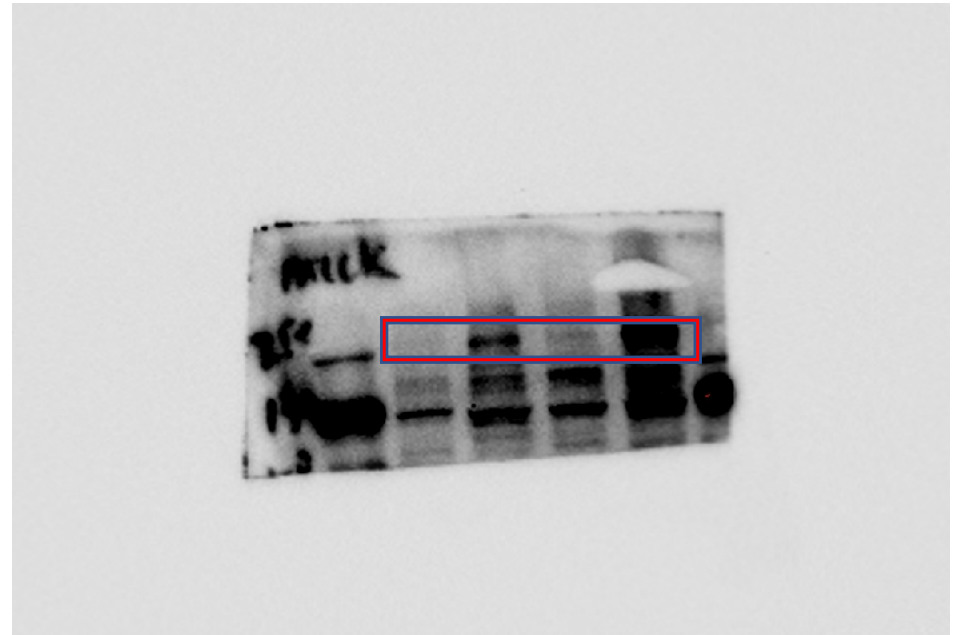
TNFR2
