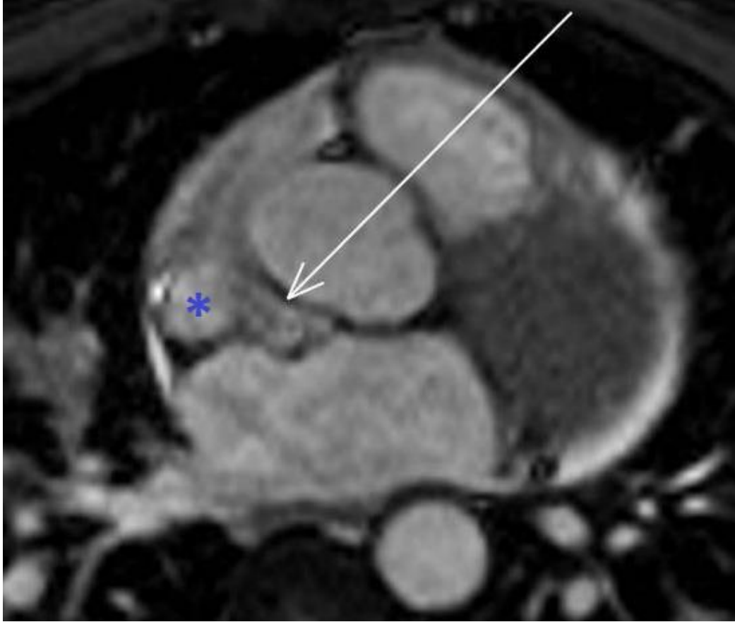
Supplemental Figure 1: RCA/SVC coronary fistula via cardiac MRI, axial. An axial slice from cardiac MRI showing the SVC (blue asterisk) and an abnormal connection (arrow).
