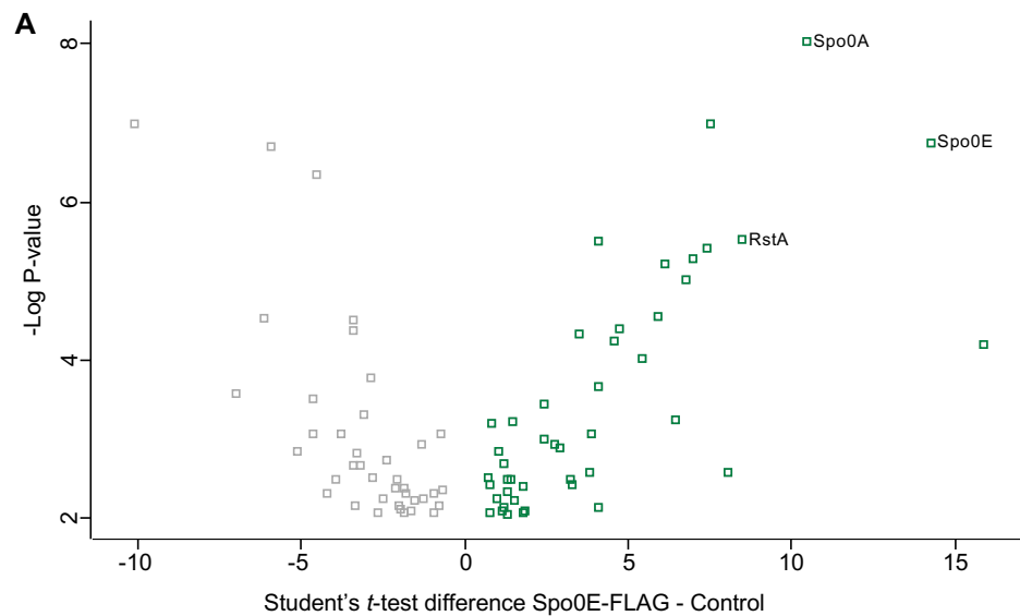
S2_Figure. Spo0E and Spo0A co-purify with regulators of sporulation, toxin, and motility. A) Scatter plot of enriched proteins identified in the Spo0E pulldown comparing the mass spec profiles of Spo0E-FLAG (MC1968, green, 45 unique proteins) and vector control (MC324, gray) and B) Spo0A pulldown comparing mass spec profiles of Spo0A-FLAG (MC1003, blue, 124 unique proteins) and vector control (MC324, gray). P \leq 0.05 . Scatter plots generated using Perseus Version 1.6.15.0.
