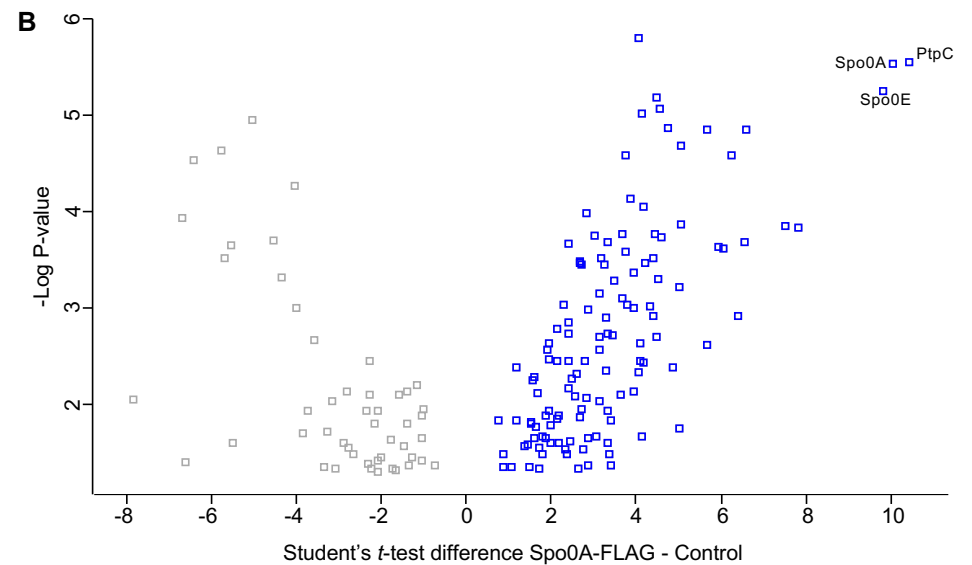
S2_Figure. Spo0E and Spo0A co-purify with regulators of sporulation, toxin, and motility. A) Scatter plot of enriched proteins identified in the Spo0E pulldown comparing the mass spec profiles of Spo0E-FLAG (MC1968, green, 45 unique proteins) and vector control (MC324, gray) and B) Spo0A pulldown comparing mass spec profiles of Spo0A-FLAG (MC1003, blue, 124 unique proteins) and vector control (MC324, gray). P \leq 0.05 . Scatter plots generated using Perseus Version 1.6.15.0.
