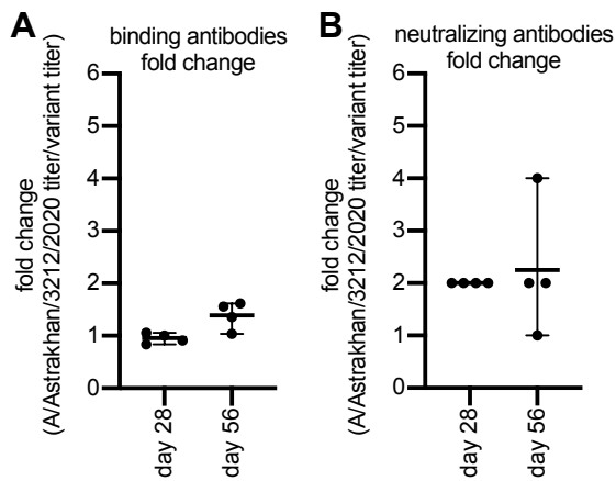
Supplementary Figure 2. Comparison of ferret antibody titers against different Clade 2.3.4.4b H5 antigens. Serum samples were collected from ferrets 28 and 56 days after vaccination. ELISA binding and neutralization titers are reported in Figure 6 . Fold change was determined by dividing antibody titers obtained using A/Astrakhan/3212/2020 antigens with titers obtained using A/pheasant/New York/22-009066-001/2022 antigens. Shown are fold change for (A) ELISA binding and (B) neutralization titers. Shown are mean and range. n=4 ferrets/group
